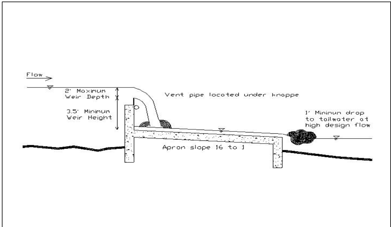
Figure 5-1. Velocity Barrier
