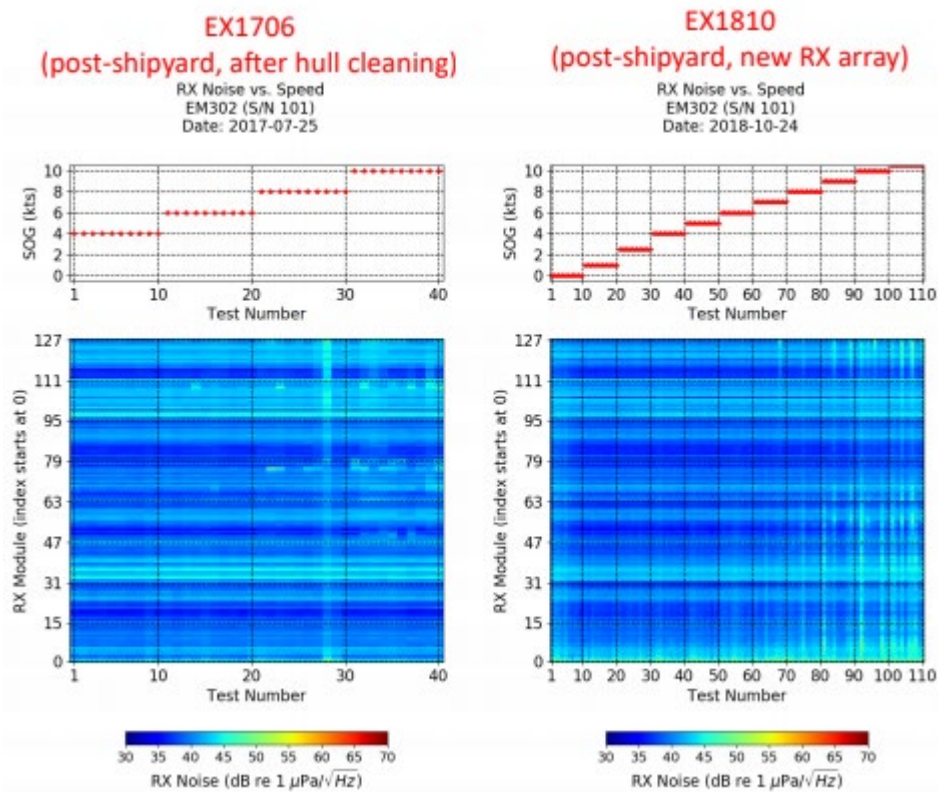
Figure 11. Comparison of RX Noise tests conducted on cruises EX-17-06 and EX-18-10.
