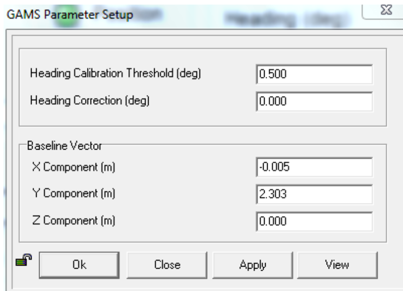
Figure 9. GAMS Parameters prior to the emergency drydock
