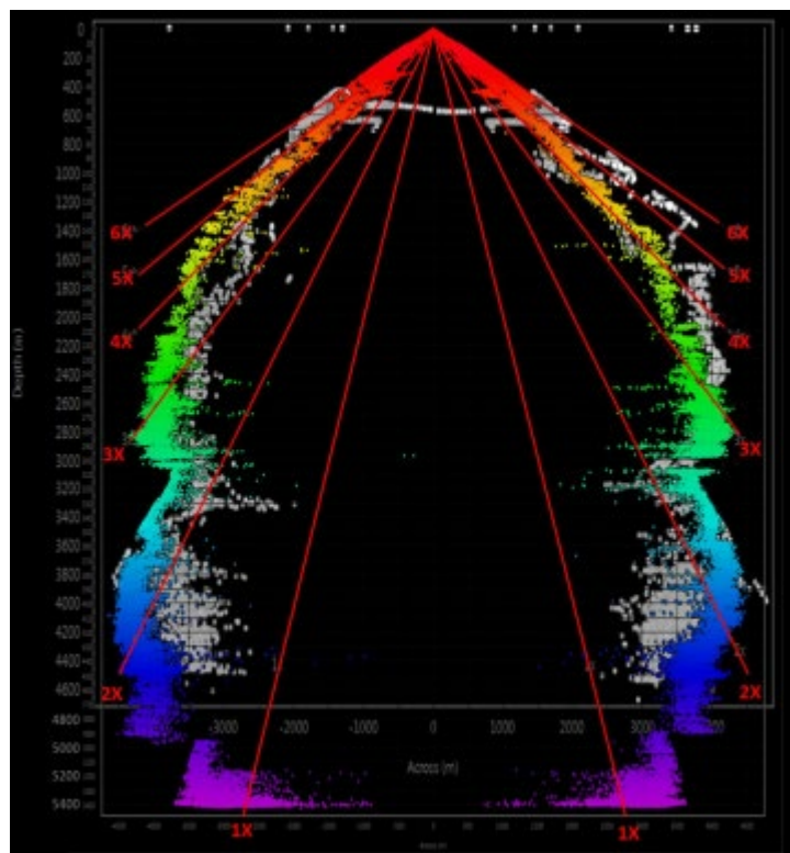
Figure 12. Swath coverage comparison between EX-17-06 (gray) and EX-18-10 (colored by depth).
