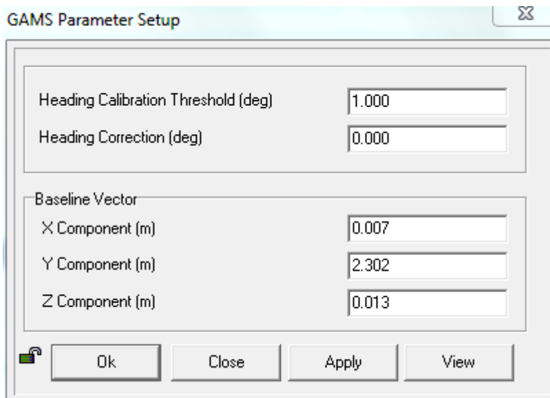
Figure 10. GAMS Parameters following the emergency drydock
