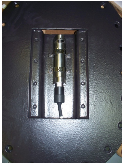
Figure 3. Photo showing the Reson SVP-70 probe attached to the access cover on the hull.
