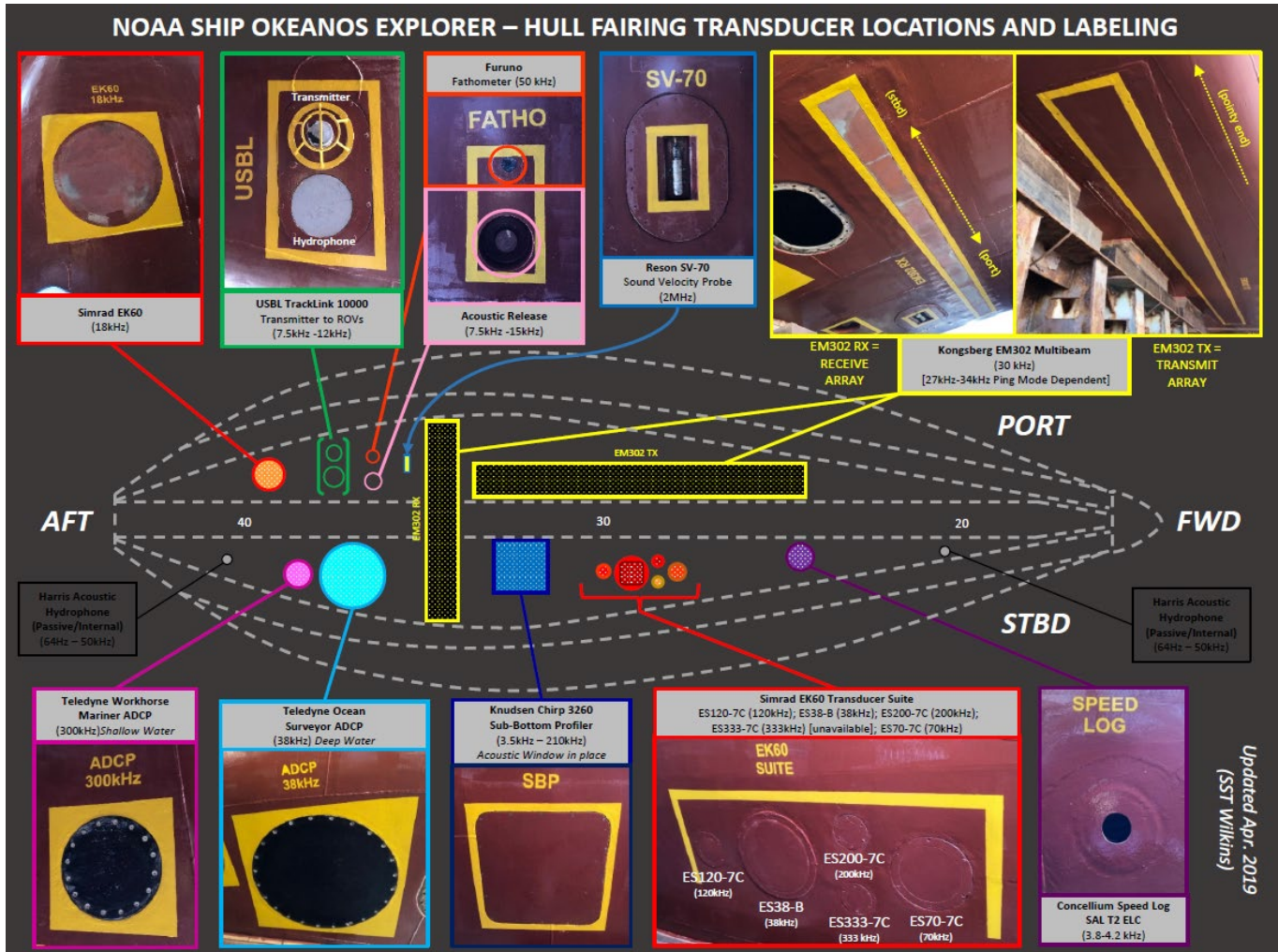
Figure 1. Sonar locations on hull. Diagram made by Senior Survey Technician Wilkins (2019).
