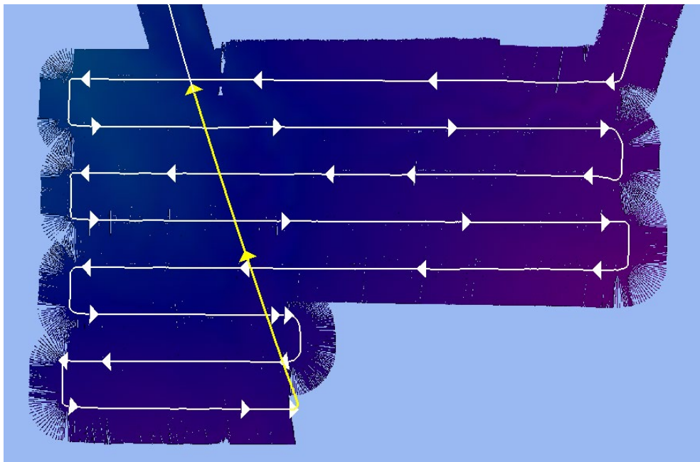
Figure 8. EX-18-02 crosslines used for cross check (Crosslines = 0177_20180404_023306_EX1802_MB.all and 0178_20180404_033306_EX1802_MB.all)
