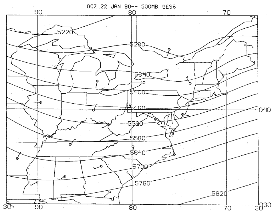
Fig. 38. NMC first-guess 500 mb heights for 0000 GMT 22 January, 1990: (a) with height residuals, (b) with wind residuals.
