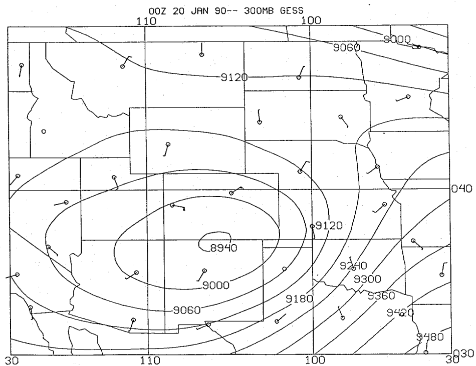
Fig. 29. NMC first-guess 300 mb heights for 0000 GMT 20 January, 1990: (a) with heights residuals, (b) with wind residuals.
