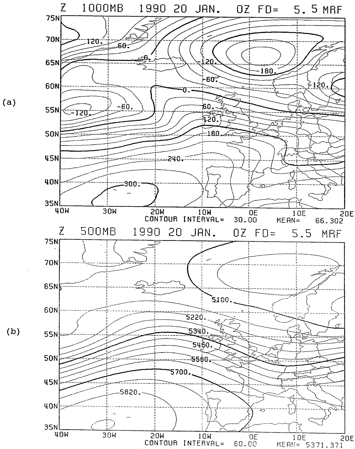
Fig. 18. NMC 5½ day height forecasts valid 1200 GMT 25 January, 1990: (a) 1000 mb, (b) 500 mb.
