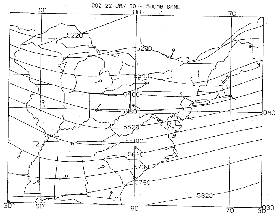
Fig. 39. NMC analysis 500 mb heights for 00Z GMT 22 January, 1990: (a) with height residuals, (b) with wind residuals.
