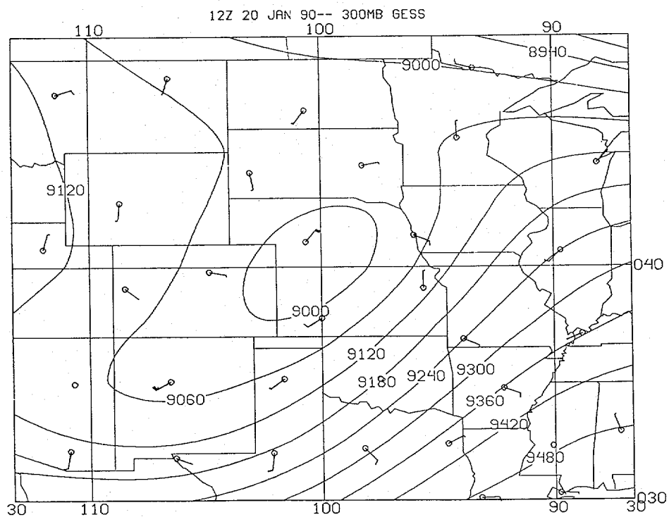
Fig. 33. NMC first-guess 300 mb heights for 1200 GMT 20 January, 1990: (a) with height residuals, (b) with wind residuals.
