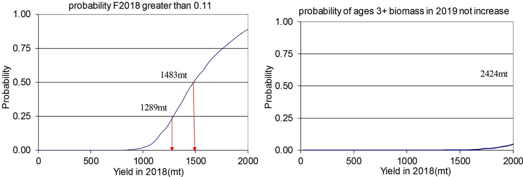
Figure 6. 2018 Projections and risks from VPA “M 0.8” results for EGB cod assuming 2017 catch at F=0.11.
