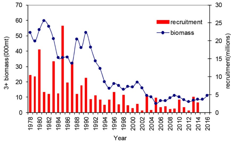
Figure 2. Biomass and recruitment for EGB cod from VPA “M 0.8”.
