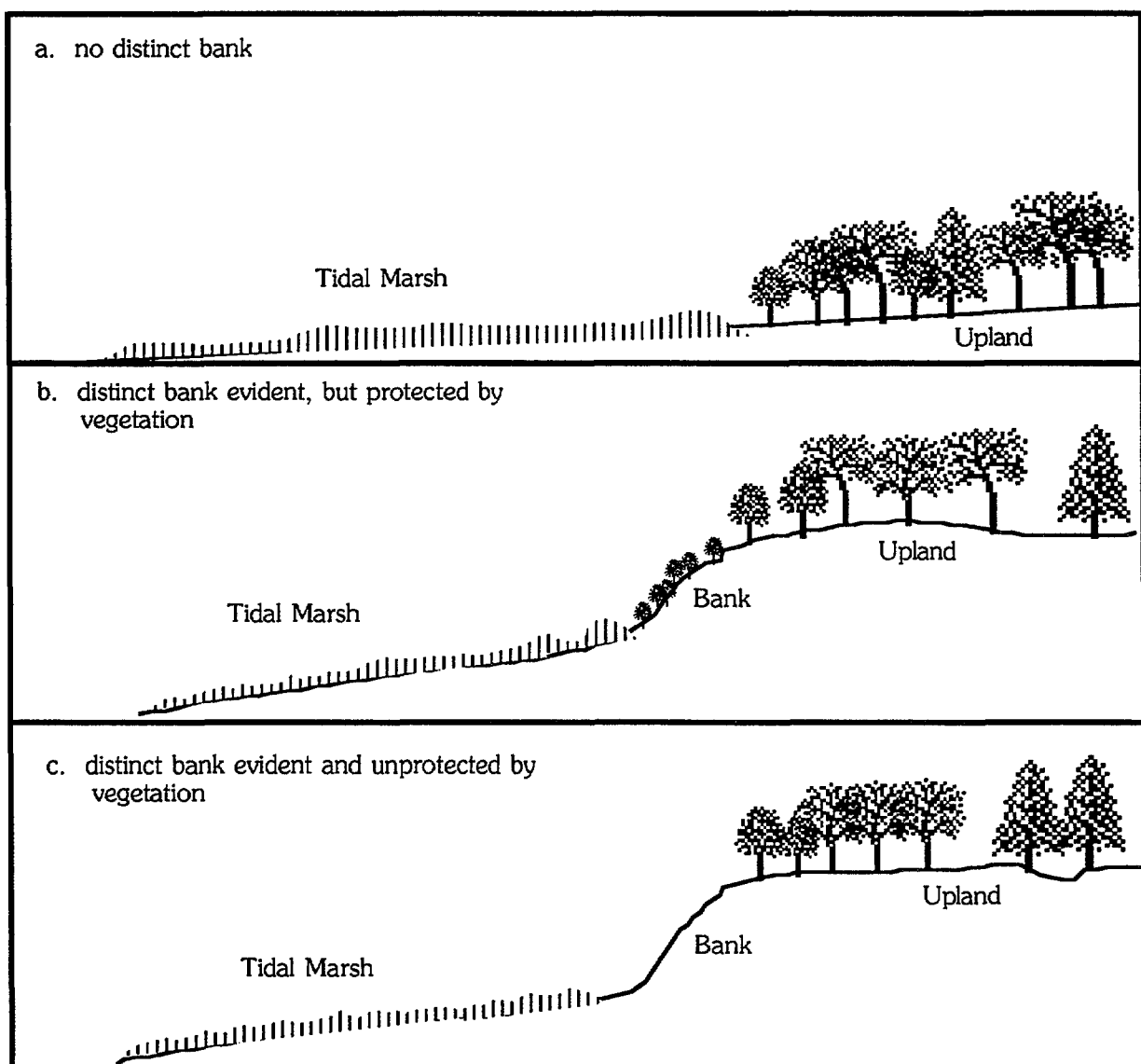
FIGURE 4-2 Wetland Morphology
