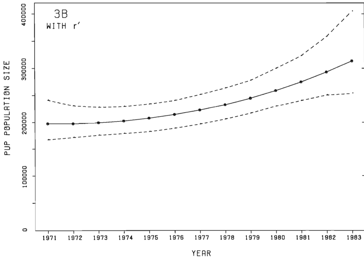
Figure 3—(a) Model estimates of pup populations for all colonies combined for the years 1971 to 1983 are shown (*) and are joined by solid straight lines. Corresponding 95% confidence intervals for these estimates are shown joined by dashed straight lines. (b) A population growth model incorporating the r' parameter (equation (10)).
