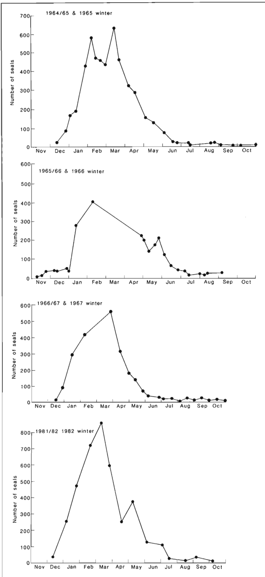
Figure 4—Annual variation in counts of all fur seals on North Head Peninsula, Macquarie Island.
