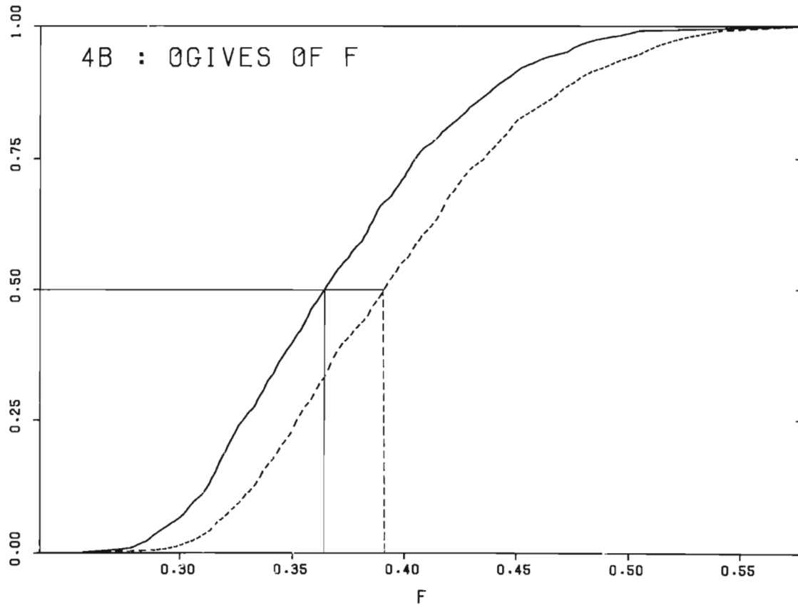
Figure 4—Probability distributions for population dynamics model parameters (a) R ; (b) F ; (c) S_a and (d) \lambda represented by ogives. The initial distributions are shown by dashed lines; the refined distributions (incorporating the equation (15) constraint) are shown by solid lines.
