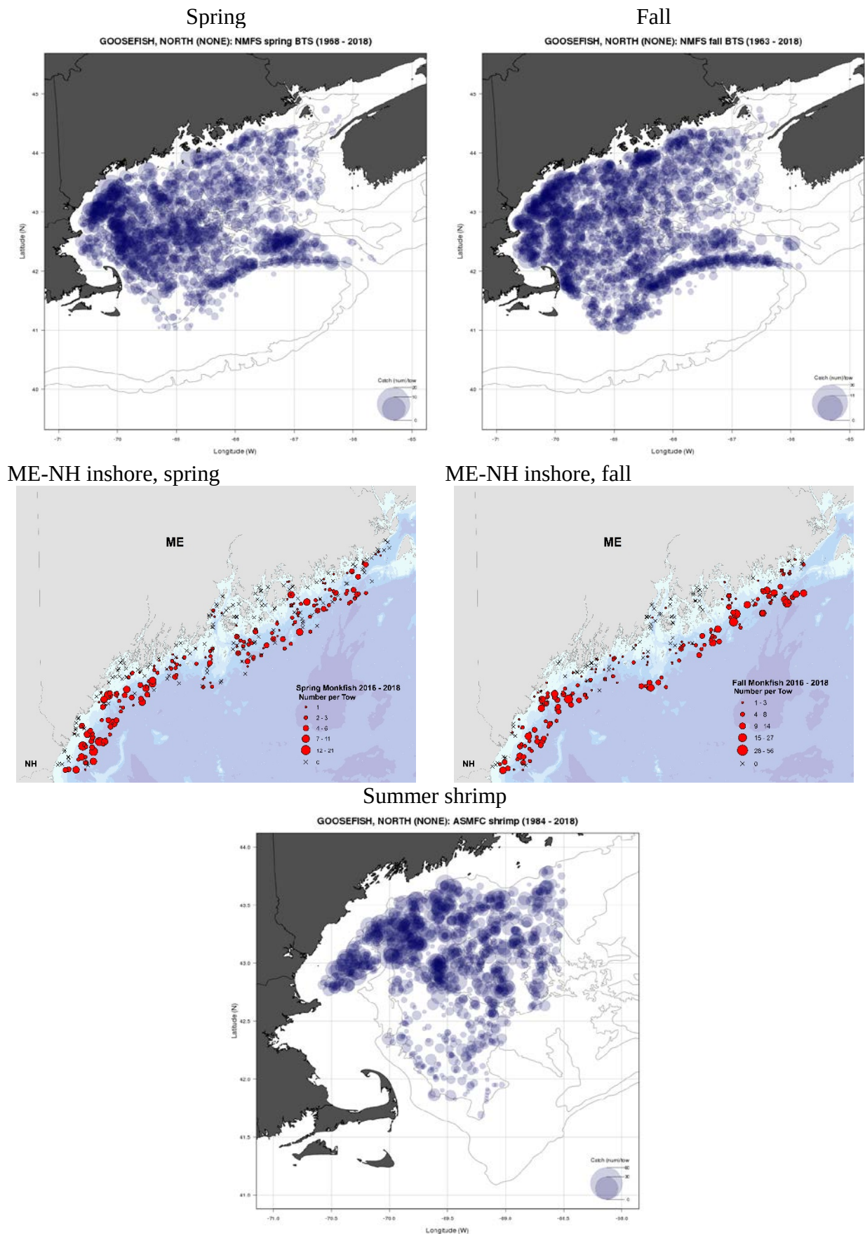
Figure D22. Distribution of monkfish in surveys in the northern management area.
