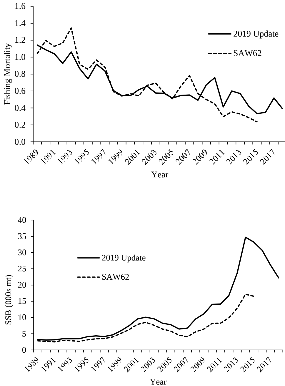
Figure A5. Historical retrospective of the 2016 (SAW 62; NEFSC 2017) and 2019 (Operational Assessment) stock assessments of black sea bass. The heavy solid lines are the 2019 Operational Assessment estimates that include the New MRIP recreational catch.
