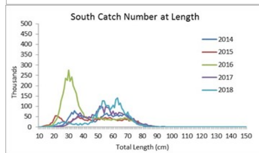
Figure D10. Length composition of monkfish commercial catch estimated using length frequency data collected by fishery observers in the southern management area.
