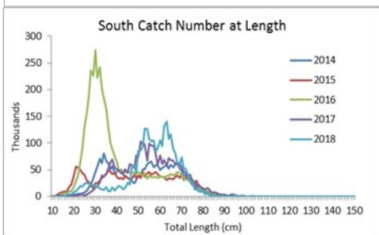
Figure D10. Length composition of monkfish commercial catch estimated using length frequency data collected by fishery observers in the southern management area.
