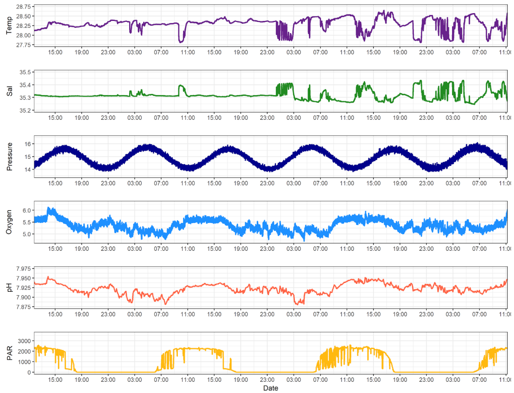
Figure 7. At Baker, the OCC team conducted a special investigation known as a “Diel Suite” that includes autonomous water samples and a variety of instrumentation that collect data over a multi-day period to quantify the diel carbonate chemistry cycle on the reef. These are the various data collected by the instrument package; water samples will be analyzed after the cruise returns.
