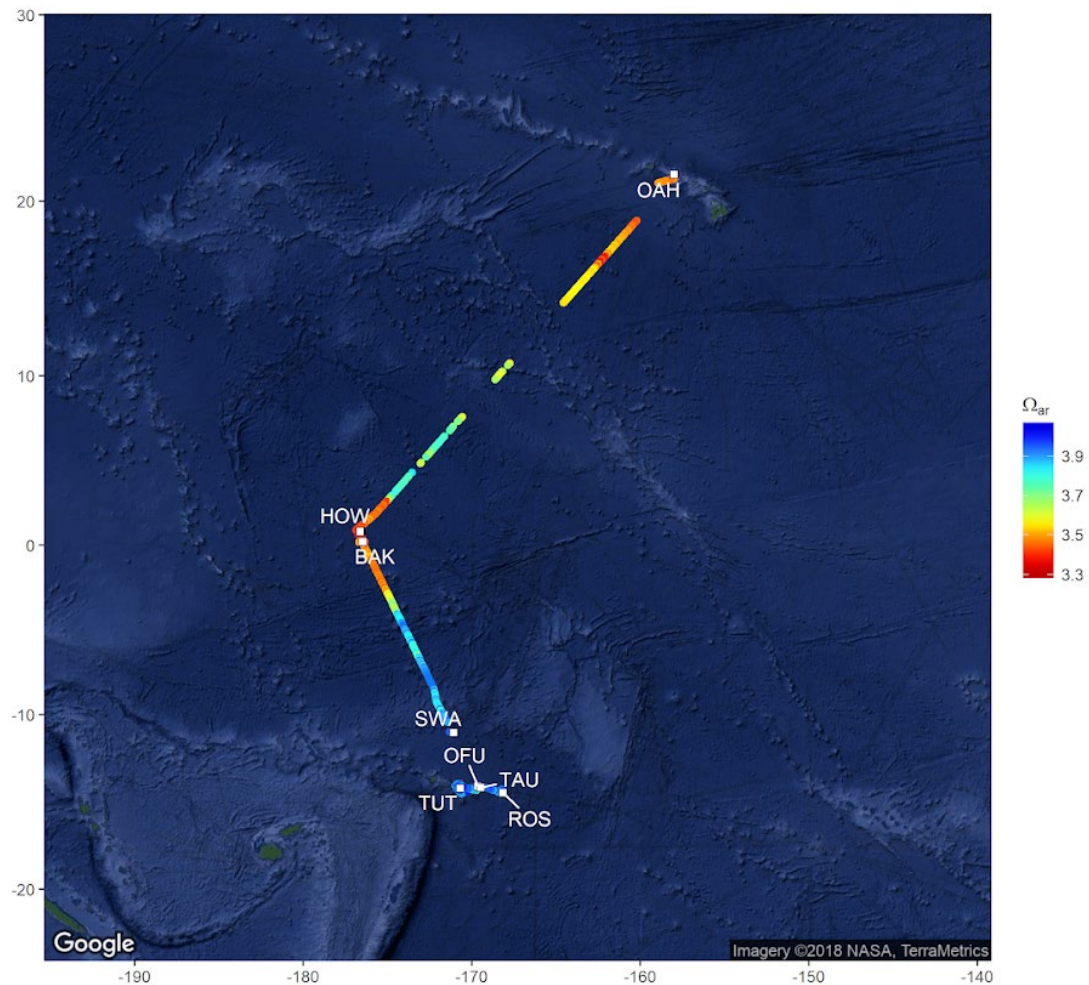
Figure 10. Spatial map of aragonite saturation state along the ASRAMP Leg 1–2 cruise track.
