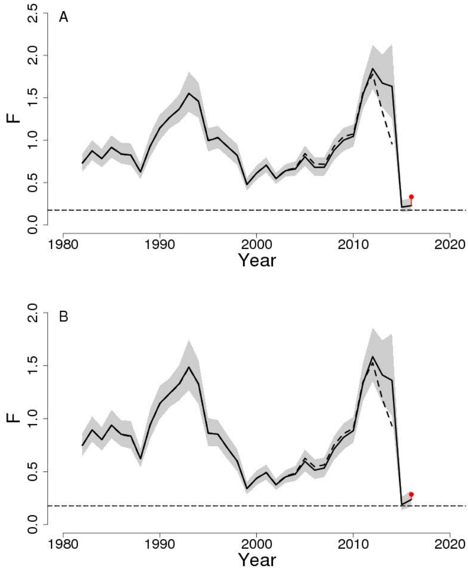
Figure 11: Estimated trends in the fully selected fishing mortality ( F ) of Gulf of Maine Atlantic cod between 1982 and 2016 from the current (solid line) and previous (dashed line) assessment and the corresponding F_{Threshold} (0.174 ( M=0.2 ), 0.177 ( M -ramp); dashed line) based on the 2017 M=0.2 (A) and M -ramp (B) assessment models. The 90% lognormal confidence intervals are shown. The red dot indicates the rho-adjusted F values that would have resulted had a retrospective adjustment been made to either model (see Special Comments section).
