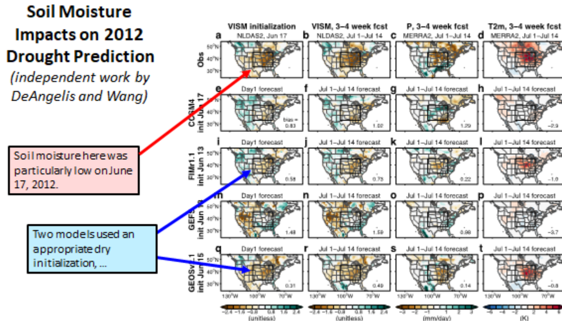
Figure 8. Impacts of land moisture initialization on drought prediction. Source: Koster brief, slide 9.
