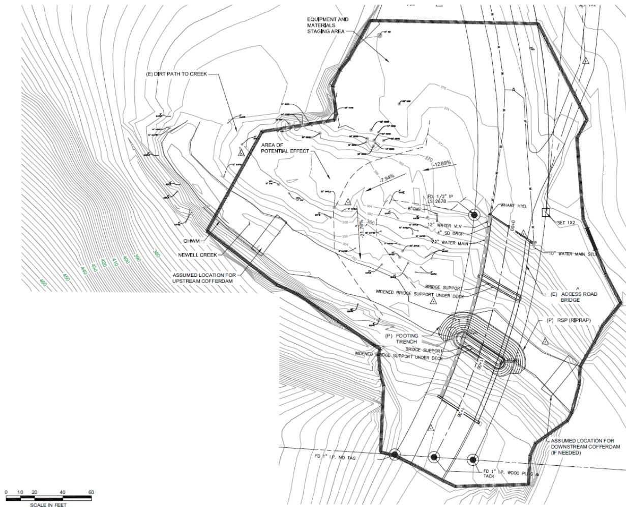
Figure 1. The Newell Creek Access Road Bridge rehabilitation project action area and general project design (Dudek 2019).
