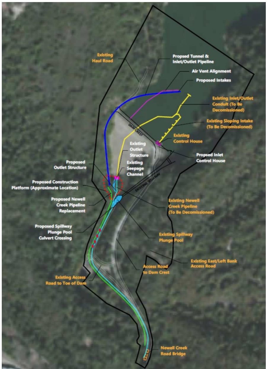
Figure 2. Map of existing and proposed project facilities/components for the Newell Creek Dam Inlet/Outlet Replacement Project. The red dots downstream of the plunge pool are the approximate locations of the existing failed log weirs proposed for replacement as part of Mitigation Project 3.
