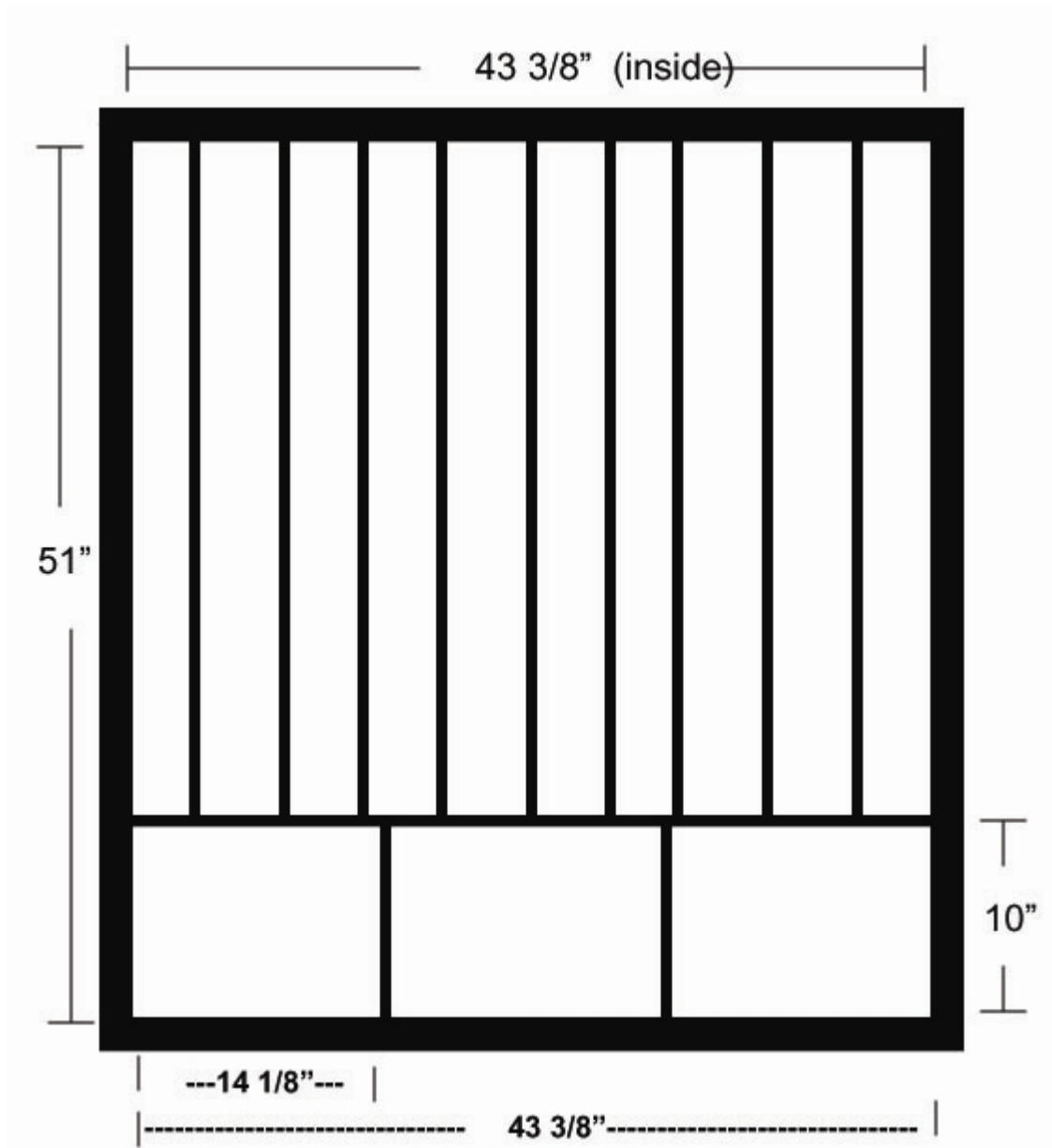
Figure 1. A diagram of the NMFS flounder TED, showing the dimensions in inches
