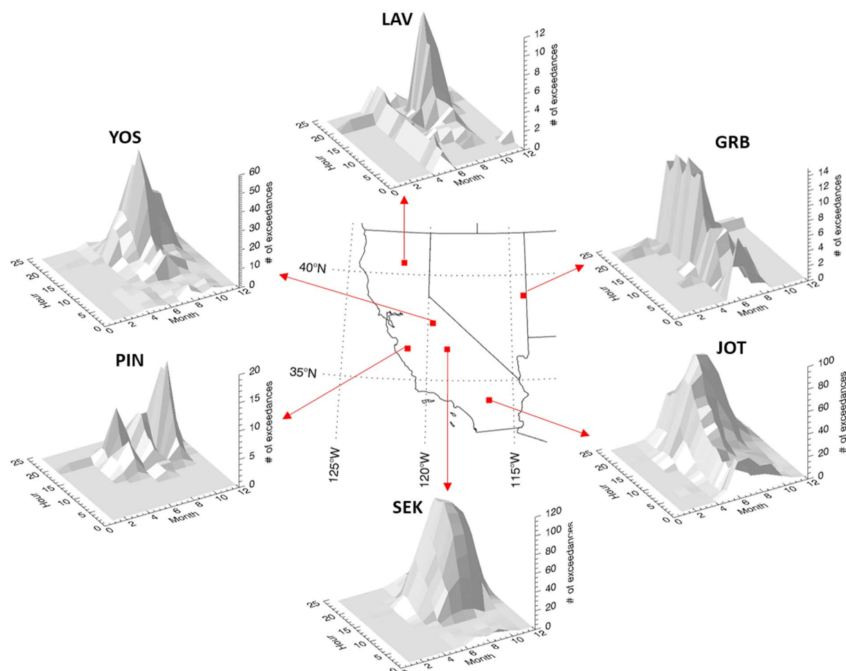
Figure 7. Frequency distributions by month and hour of day for the number of times hourly \text{O}_3 mixing ratios exceed 70 ppb during 2010–2014 at Great Basin (GRB, elev. 2,060 m), Joshua Tree (JOT, elev. 1,224 m), Sequoia (SEK, elev. 1,225 m), Pinnacles (PIN, elev. 335 m), Yosemite (YOS, elev. 1,605 m), and Lassen Volcanic (LAV, elev. 1,756 m) National Parks.
