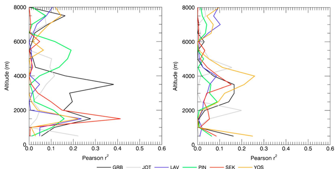
Figure 8. Correlation coefficients of mean AJAX \text{O}_3 with seasonally corrected surface \text{O}_3 measured at Great Basin (GRB, black), Joshua Tree (JOT, gray), Lassen Volcanic (LAV, blue), Pinnacles (PIN, green), Sequoia (SEK, red), and Yosemite (YOS, orange) National Parks in spring (April–May, left) and summer (June–September, right) 2010–2014.
