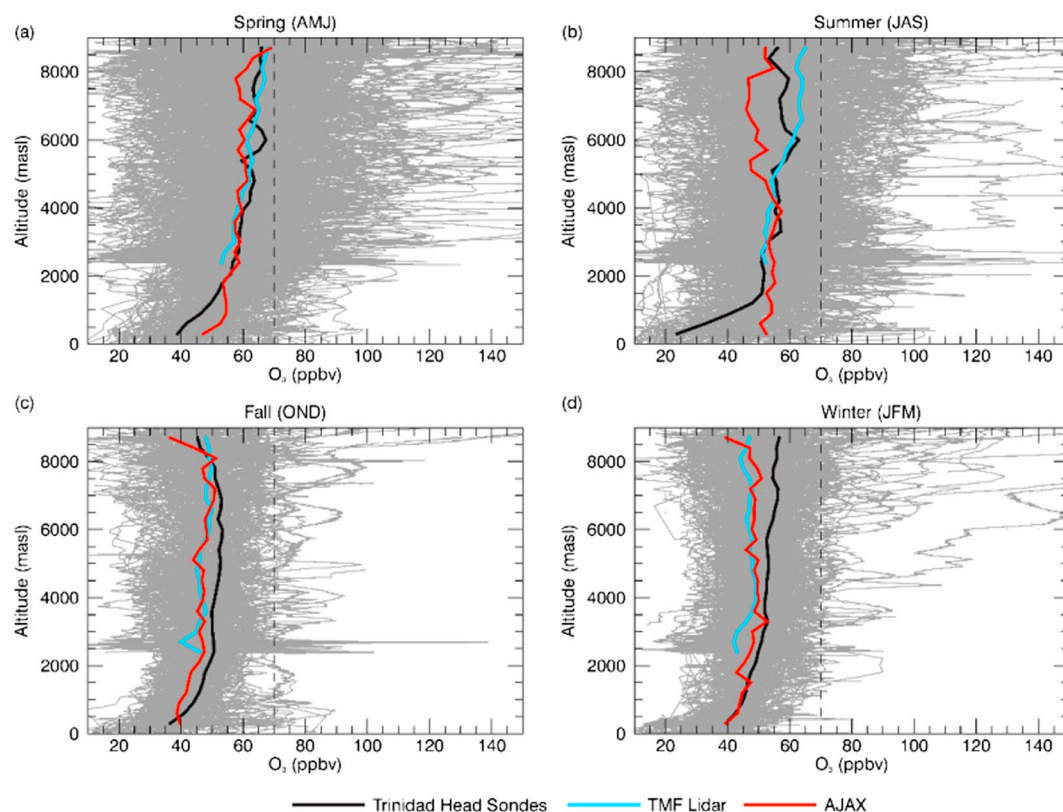
Figure 5. Seasonal O_3 profiles (January 2011 to December 2015) during (a) spring (April, May, June (AMJ)), (b) summer (July, August, September (JAS)), (c) fall (October, November, December (OND)), and (d) winter (January, February, March (JFM)). Bold lines highlight the seasonal averages from aircraft (AJAX, red), ozonesonde (Trinidad Head, black), and the lidar (Table Mountain, blue). The black dashed vertical lines indicate the 70 ppbv NAAQS. The gray lines present all O_3 data measured by AJAX, ozonesonde, and lidar (Note: Lidar data cover January 2012 to July 2015).
