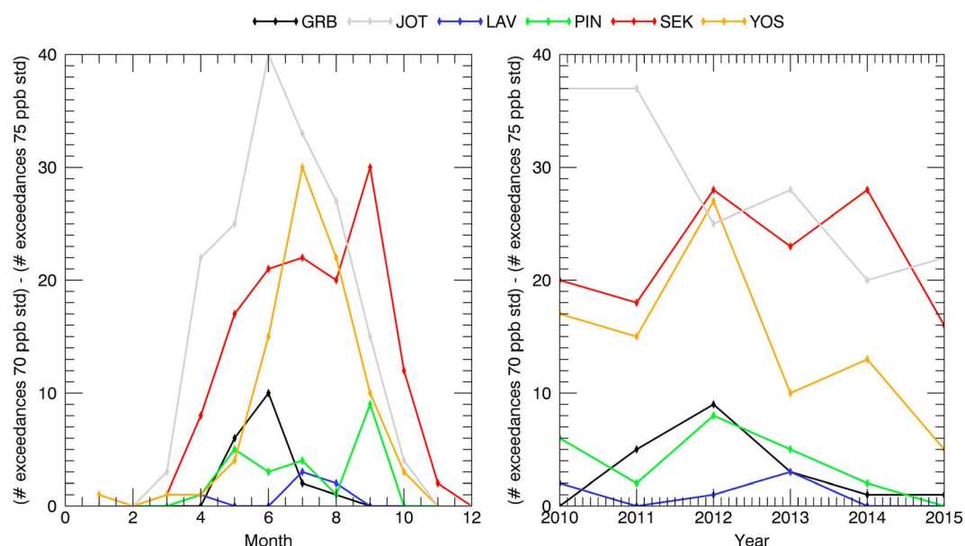
Figure 4. Assessing the impact of the reduced NAAQS on the number of O_3 exceedances during 2010–2015 by (left) month and (right) year at Great Basin (GRB, black), Joshua Tree (JOT, gray), Lassen Volcanic (LAV, blue), Pinnacles (PIN, green), Sequoia (SEK, red), and Yosemite (YOS, orange) National Parks (the total number of exceedances of 70 ppb standard minus the total number of exceedances of 75 ppb standard for 2010–2015).
