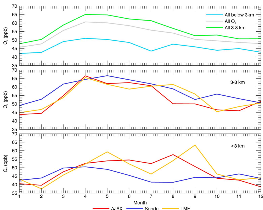
Figure 6. January 2011 to December 2015 averaged seasonal O_3 cycle of combined measurements by AJAX (red), ozone-sonde (blue), and the tropospheric lidar (TMF, orange) at (middle) 3–8 km and (bottom) below 3 km. (top) The monthly averages of all the data from surface to 8 km (gray), between 3 and 8 km (green, free troposphere), and below 3 km (blue, boundary layer).
