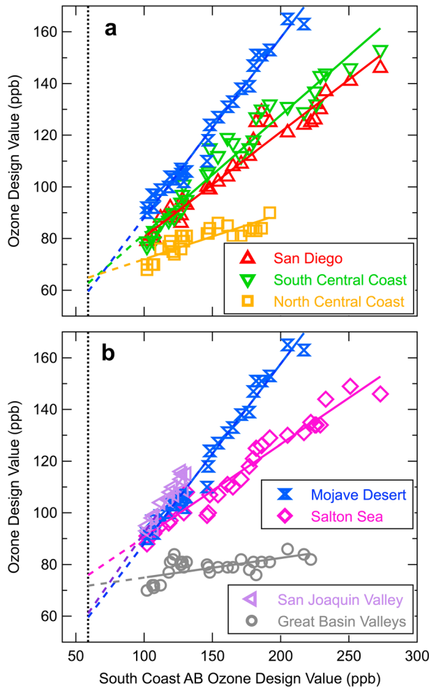
Figure 4. Correlations of ODVs between Southern California air basins and the South Coast Air Basin. The solid lines indicate linear regressions to the symbols. The dashed lines are extrapolations of the linear fits to the y_0 value = 58.9 ppb determined for the South Coast Air Basin (vertical dotted line).
