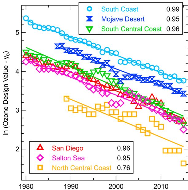
Figure 3. Evolution of the natural logarithm of the ODV enhancement above y_0 over the past 36 years in six Southern California air basins. The straight lines indicate linear regression fits to the symbols, with the r^2 of those fits indicated in the annotations.
