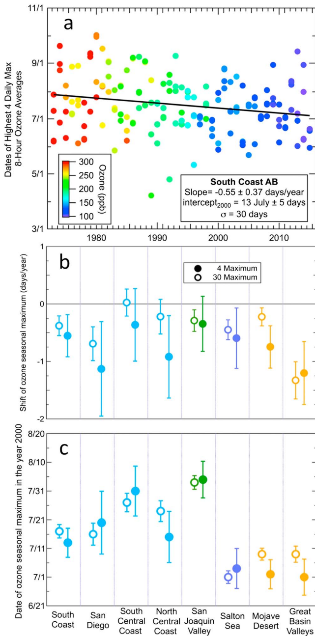
Figure 7. Evolution of the dates of occurrence of the highest maximum daily 8 h average (MDA8) ozone concentrations over the past 42 years in the Southern California air basins. (a) The symbols indicate the dates that the four highest maxima were recorded in the South Coast Air Basin each year and are color-coded according to the ozone concentration. The solid line gives the linear regression fit to the symbols; slopes and intercepts with 95% confidence limits and the root-mean-square deviation from the fit are annotated. Comparison of (b) rate of change of ozone seasonal maximum and (c) the date of the seasonal maximum in the year 2000 in the eight Southern California air basins. The results for the 4 (closed symbols) and the 30 (open symbols) highest MDA8 concentrations in each year are shown with 95% confidence limits.
