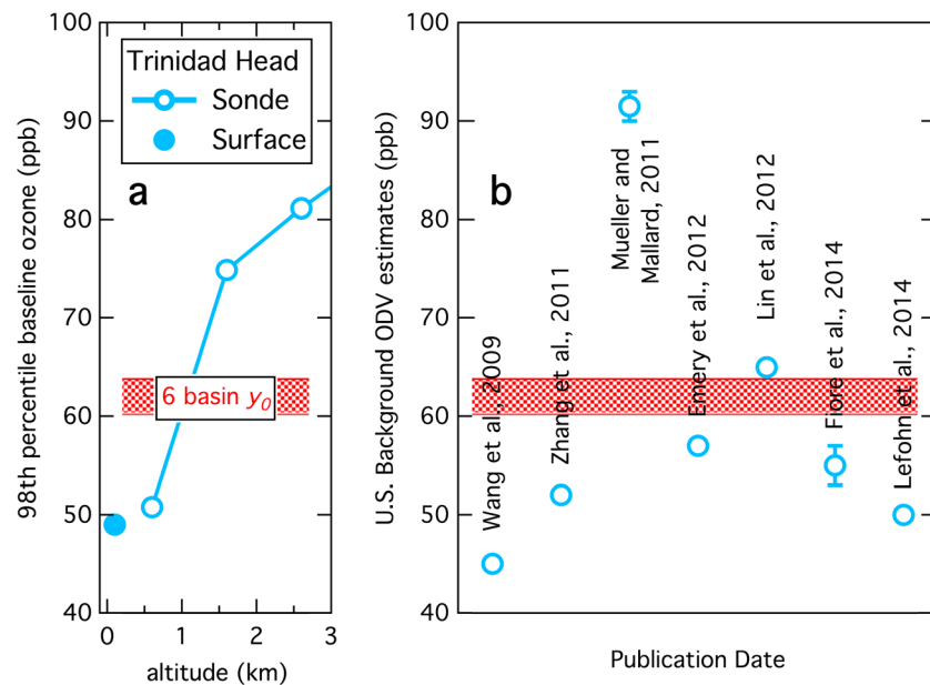
Figure 6. Comparison of y_0 determined for six air basins with (a) the 98th percentile of the baseline ozone concentrations measured at Trinidad Head in May through September and (b) estimates of the U.S. background ODV from modeling studies. The red hatched bar indicates the six basin y_0 \pm confidence limits in both plots. In Figure 6a the solid symbol gives the Trinidad Head surface result and the open symbols give the results from the sonde data (also included in Figure 1) averaged over 1 km thick layers beginning at 0.1 km. The symbols in Figure 6b give the results from model calculations estimated from the indicated literature references (Wang et al., 2009; Zhang et al., 2011; Mueller & Mallard, 2011; Emery et al., 2012; Lin et al., 2012; Fiore et al., 2014; Lefohn et al., 2014); Section S1 in the supporting information gives details of the interpretation of these model results.
