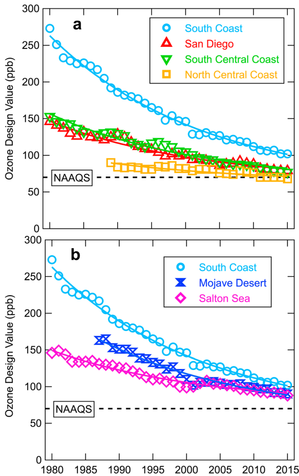
Figure 2. Evolution of the ozone design values over the past 36 years in (a) the four Southern California coastal air basins and (b) two inland air basins with the South Coast included for comparison. The symbols give the annual ODVs for each air basin, and the solid curves indicate the fits of Equation (1) to the corresponding ODVs. The dashed line indicates the 2015 NAAQS.
