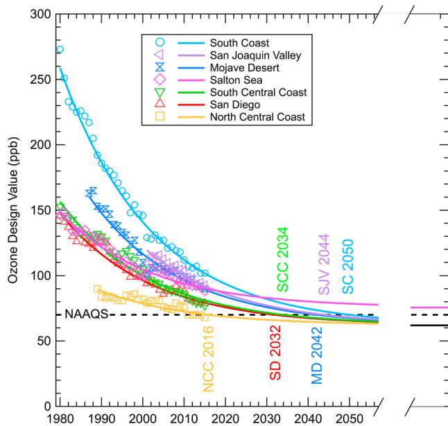
Figure 8. Past and projected evolution of the basin ozone design values in seven Southern California air basins. The symbols give the annual ODVs for each air basin, and the solid curves indicate the fits of equation (1) with the parameters from Table 4 to the corresponding ODVs with projections to the year 2058. The line segments at right indicate the asymptotes (i.e., the parameter y_0 ) toward which the ODVs are converging (six basins to a common value in black, and the Salton Sea Air Basin approaching its own limit in its corresponding color). The dashed line indicates the NAAQS. The six annotated years in the colors with initials corresponding to the respective basins indicate the projected date that the basin ODV will drop to the NAAQS.
