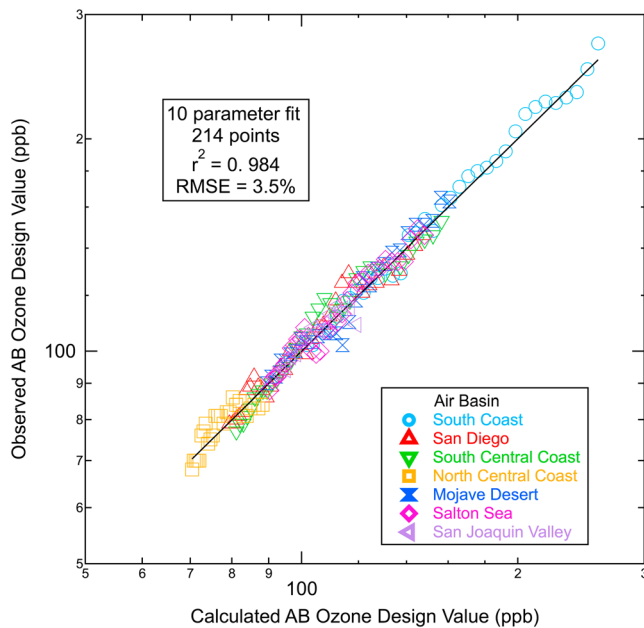
Figure 5. Comparison of observed ODVs with those calculated from equation (1) based upon a multivariate regression with 10 parameters for seven air basins (Table 4). The solid line indicates the 1:1 relationship. The total number of data points, the square of the correlation coefficient for the log-transformed data, and the root-mean-square relative deviations of the calculated ODVs are indicated.
