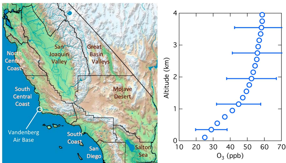
Figure 1. Map of the eight Southern California air basins and plot of the vertical profile of baseline ozone concentrations measured by 471 ozone sondes released at Trinidad Head, a Northern California coastal site (Oltmans et al., 2008) during the 5 month (May–September) ozone season from 1997 through 2014. The symbols show averages over 200 m altitude increments with error bars giving example standard deviations.
