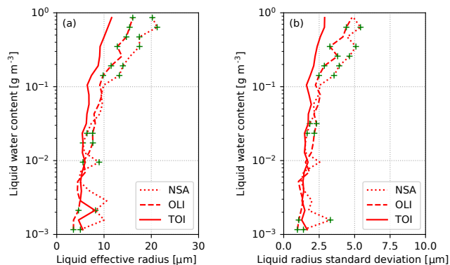
Figure 5. (a) Mean r_{\text{eff}} and (b) mean SD as a function of LWC for the data presented in Fig. 4. The green crosses indicate a significant difference between OLI and NSA (5 % confidence interval).
