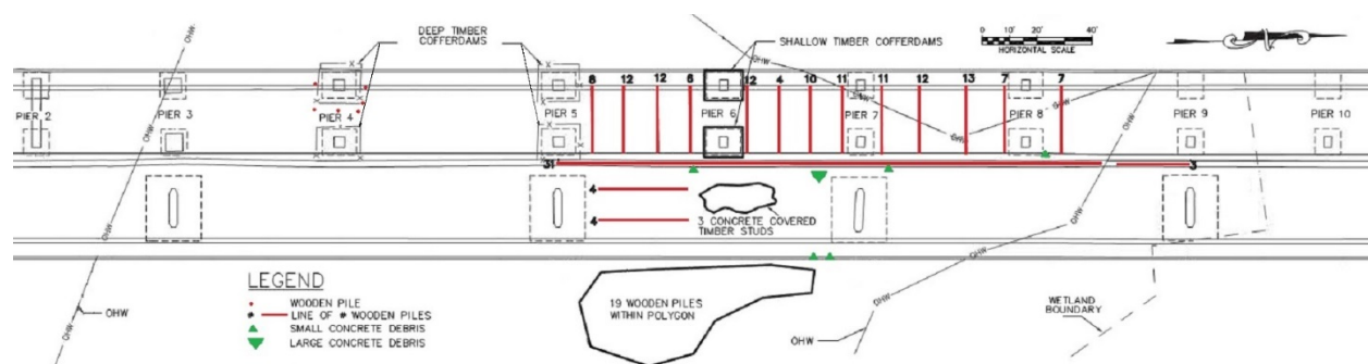
Figure 4. Overhead drawing of the existing Sammamish River Bridges showing the locations of derelict timber piles and cofferdams and concrete debris that would be removed during Year-2 work. The red lines indicate lines of piles to be removed. The number at the end of each line indicates the number of piles in the line. The green triangles indicate areas of concrete debris. The 6 red dots at pier 4 indicate individual piles (Adapted from Figure 5 in Jacobs 2018b).
