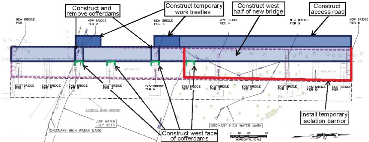
Figure 2. Overhead drawing of the Sammamish River Bridges relative to the ordinary high water line and the 2015 low water line, showing planned Year-1 construction. The dashed magenta outline shows the footprint of the new West Bridge. The light blue rectangle indicates the western half of the new bridge. The darker blue rectangles indicate the temporary access road and trestles. The 3-sided red line indicates the temporary isolation barrier. (Adapted from Figure 4 in Jacobs 2016).
