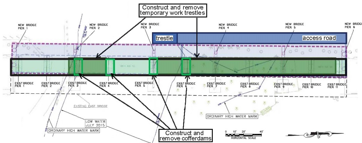
Figure 3. Overhead drawing of the Sammamish River Bridges relative to the ordinary high water line and the 2015 low water line, showing planned Year-2 construction. The dashed magenta outline shows the footprint of the new West Bridge. The light and dark green rectangles outlined in black indicates the eastern half of the new bridge. The darker green rectangles indicate the locations of temporary trestles. (Adapted from Figure 5 in Jacobs 2016).
