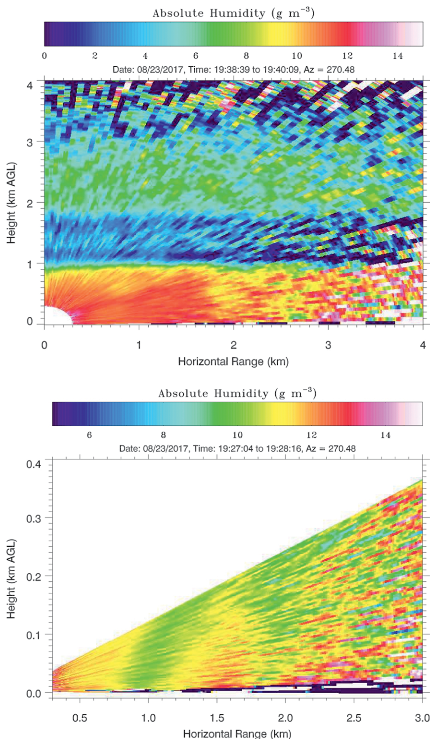
FIG. 8. Alternating RHI scans of the UDIAL for studying the 2D water vapor field performed during IOP11 on 23 Aug 2017. (top) The 0°–90° RHI with scan speed of 1^\circ \text{ s}^{-1} and a range resolution of 200 m showing several turbulent eddies from the surface up to the PBL top at approximately 900 m AGL. (bottom) The 0°–7° RHI with scan speed of 0.1^\circ \text{ s}^{-1} and also a range resolution of 200 m revealing several coherent structures in the surface water vapor field with an amplitude of \approx 2 \text{ g m}^{-3} ranging from turbulent to mesogamma scales.
