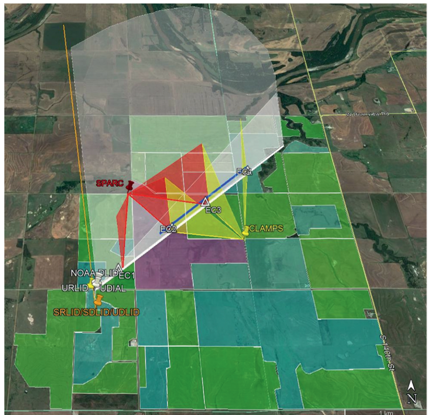
FIG. 4. The deployment and scanning strategy for LAFE at the ARM SGP central facility. The three scanning lidar systems (UDIAL, URLID, and NOAA DLID) were located 300 m north of the SRL and scanning in elevation above the main RHI (thick white line and planes). Four energy balance stations (including soil moisture and temperature) were installed at the tower locations 1–4 (EC1–4). Dual-Doppler lidar scans were also performed at these tower locations using a combination of the NOAA DLID and the DLIDs included with the SPARC (red planes) and CLAMPS (yellow planes). The sUAS flight track (blue) was parallel to the main RHI path. The field types are indicated by color: pasture (cyan), farm fields (which were mainly wheat stubble or soybeans; green), and conservation research program land (which has native grasses that are about 0.6 m tall; purple).
