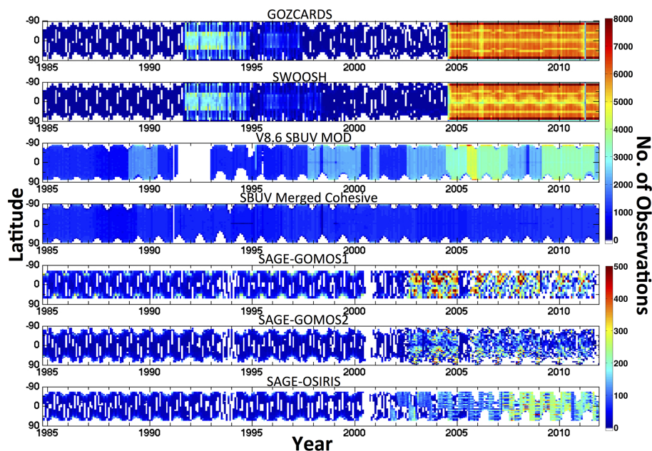
Figure 2. Latitudinal availability of data over the 1984–2011 period. The colours represent the sum of measurements used per latitudinal grid box over the entire profile for each merged data set (note that two separate colour scales are used).
