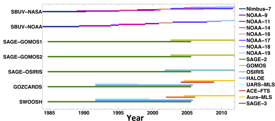
Figure 1. Time coverage of the individual instruments used in each of the seven data sets considered in this study for the 1984–2011 period.
