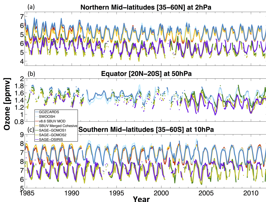
Figure 4. Monthly mean ozone (ppmv) in (a) the Northern Hemisphere mid-latitudes ( 35\text{--}60^\circ\text{N} ) at 2 hPa, (b) the tropics ( 20^\circ\text{N}\text{--}20^\circ\text{S} ) at 50 hPa, and (c) the Southern Hemisphere mid-latitudes ( 35\text{--}60^\circ\text{S} ) at 10 hPa. Note that the data sets are separated in the two mid-latitude plots (a) and (c) for clarity, and thus the y-axis values are shifted.
