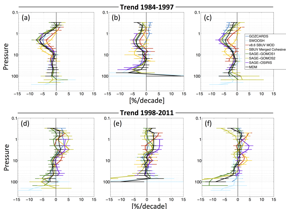
Figure 8. Latitudinal average ozone profile trends (in \% \text{ decade}^{-1} ) for 1984–1997 (top row) and 1998–2011 (bottom row). Left column ( a and d ): Southern Hemisphere mid-latitudes ( 35\text{--}60^\circ \text{S} ); middle column: ( b and e ) tropics ( 20^\circ \text{N--}20^\circ \text{S} ); right column: ( c and f ) Northern Hemisphere mid-latitudes ( 35\text{--}60^\circ \text{N} ). The horizontal error bars indicate \pm 2\sigma uncertainties.
