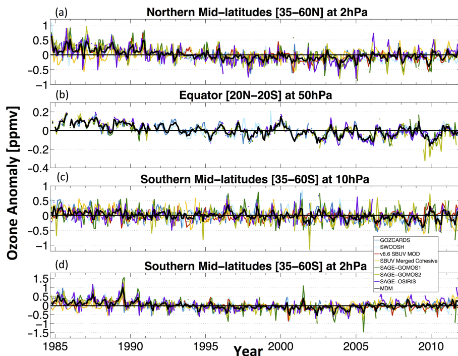
Figure 6. Monthly mean anomalies for (a) the Northern Hemisphere mid-latitudes ( 35\text{--}60^\circ\text{N} ) at 2 hPa, (b) the tropics ( 20^\circ\text{N}\text{--}20^\circ\text{S} ) at 50 hPa, and (c) the Southern Hemisphere mid-latitudes ( 35\text{--}60^\circ\text{S} ) at 10 hPa. Note the different y-axis ranges for each plot (a)–(d).
