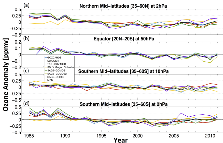
Figure 7. Annual mean anomalies for (a) the Northern Hemisphere mid-latitudes ( 35\text{--}60^\circ\text{N} ) at 2 hPa, (b) the tropics ( 20^\circ\text{N}\text{--}20^\circ\text{S} ) at 50 hPa, and (c) the Southern Hemisphere mid-latitudes ( 35\text{--}60^\circ\text{S} ) at 10 hPa. Annual averages are only shown if data for more than 7 of 12 months per year were available. Note the different y-axis ranges.
