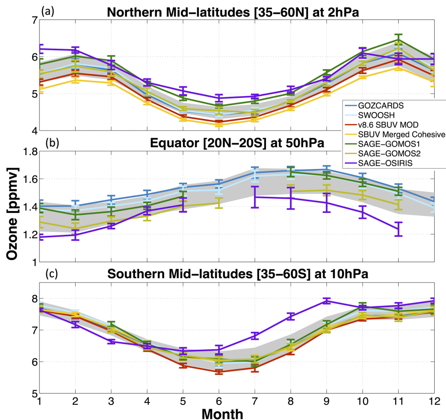
Figure 3. Annual cycle averaged over the 1984–2011 period for (a) the Northern Hemisphere mid-latitudes ( 35\text{--}60^\circ\text{N} ) at 2 hPa, (b) the tropics ( 20^\circ\text{N}\text{--}20^\circ\text{S} ) at 50 hPa, and (c) the Southern Hemisphere mid-latitudes ( 35\text{--}60^\circ\text{S} ) at 10 hPa. Error bars indicate \pm 2 standard errors of the mean, while the grey range shows \pm 1 standard deviation (mean of all data sets). Values (monthly values, standard deviation, and standard error) are shown only if data are available for more than half (14) of the 28 years in the time series.
