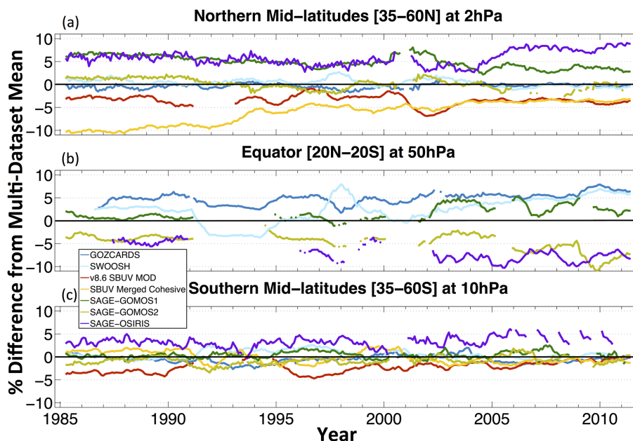
Figure 5. Monthly mean percentage differences from the multi-data-set mean (MDM; see text for details) for (a) the Northern Hemisphere mid-latitudes ( 35\text{--}60^\circ\text{N} ) at 2 hPa, (b) the tropics ( 20^\circ\text{N--}20^\circ\text{S} ) at 50 hPa, and (c) the Southern Hemisphere mid-latitudes ( 35\text{--}60^\circ\text{S} ) at 10 hPa.
