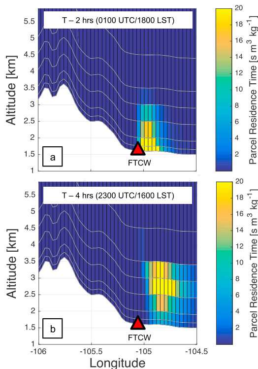
Figure 9. Vertical distribution of parcel concentration along 40.6N (east-west through northern Colorado) output from the FLEXPART back trajectory calculation at (a) 0100 UTC (1800 LST) and (b) 2300 UTC (1600 LST 22 July 2014). One hundred parcels were released at the FTCW site between 0200 and 0300 UTC (2000 LST). Higher residence times indicate that more parcels spend more time in a grid cell.
