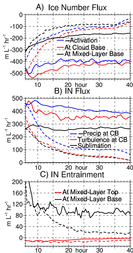
Figure 9. Horizontally averaged fluxes from the Control and NoRecycle integrations for hours 6–40 (smoothed with 90 min running average). NoRecycle shown with dashed lines. (a) N_{ICE} flux at cloud base due to turbulence+subsidence+precipitation (red), mixed-layer base due to turbulence+subsidence+precipitation (black), and due to activation (multiplied by -1 , blue), in units of \text{mL}^{-1} \text{h}^{-1} . (b) N_{IN} flux at cloud base (indicated by CB in legend) due to turbulence (red), N_{IN} flux due to sublimation (black), and precipitation of N_{ICE} at cloud base (multiplied by -1 , blue), in units of \text{mL}^{-1} \text{h}^{-1} . (c) N_{IN} entrainment at mixed-layer top (red) and base (black), in units of \text{mL}^{-1} \text{h}^{-1} .
