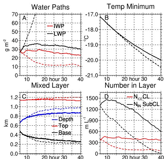
Figure 8. Control and NoRecycle time series for hours 6–40 (smoothed with 9 min running average). NoRecycle shown with dashed lines. (a) LWP (black) and IWP (red), in units of g m^{-2} . (b) Minimum horizontally averaged temperature in the column, in units of ^{\circ}C . (c) Mixed-layer depth (blue), top height (red), and base height (black), in units of km. (d) N_{ICE} integrated over cloud layer (referred to as CL, red) and N_{IN} integrated over subcloud layer (referred to as SubCL, black), in units of mL^{-1} .
