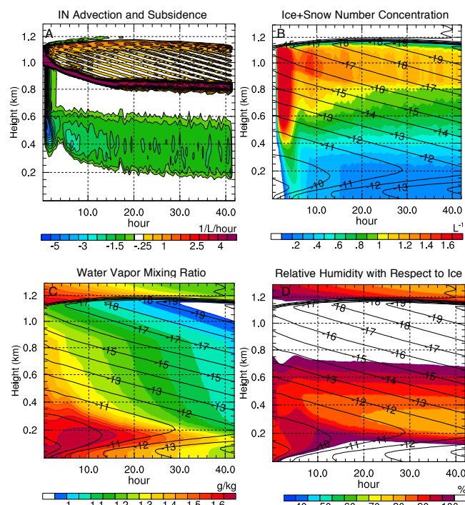
Figure 7. Time–height cross sections of horizontally averaged (a) IN advection plus subsidence, in units of L^{-1} h^{-1} ; (b) ice plus snow number concentration, in units of L^{-1} ; (c) water vapor mixing ratio, in units of g kg^{-1} ; and (d) relative humidity with respect to ice, in units of percent, from CNT simulation. Temperature, in units of ^{\circ}C , shown with black contour lines in (b, c, d).
