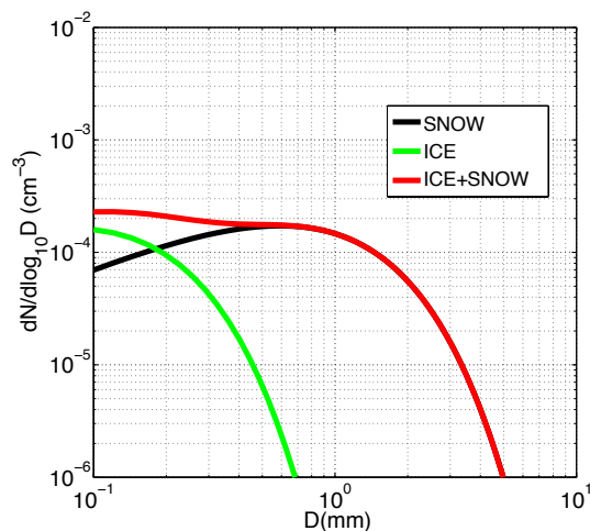
Figure 5. Simulated ice particle number size distributions using in-cloud mass and number concentrations. Ice water mixing ratio = 3e-4 \text{ g kg}^{-1} , ice number concentration = 0.4 \text{ L}^{-1} , snow water mixing ratio = 2.4e-2 \text{ g kg}^{-1} , and snow number concentration = 0.45 \text{ L}^{-1} .
