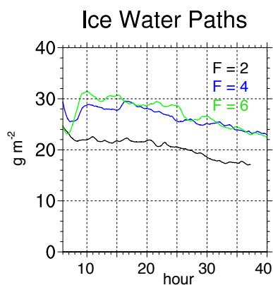
Figure 3. Sensitivity of ice water path to the parameter F in Eq. (2). Note the similar ice water paths for F = 4 and F = 6 (total N_{\text{IN}} initial values of 5.8 and 8.7 \text{ L}^{-1} , respectively).
