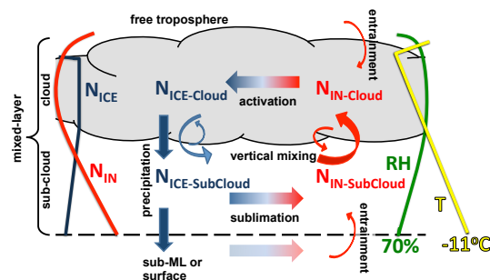
Figure 10. Schematic of feedback loops that maintain ice production and the phase partitioning between cloud liquid and ice in an AMPS. Red denotes N_{IN} . Blue denotes N_{ICE} . The size of the arrow indicates the relative magnitude of the flux. Vertical profiles of N_{ICE} , N_{IN} , relative humidity, and temperature shown with thin blue, red, green, and yellow lines, respectively.
