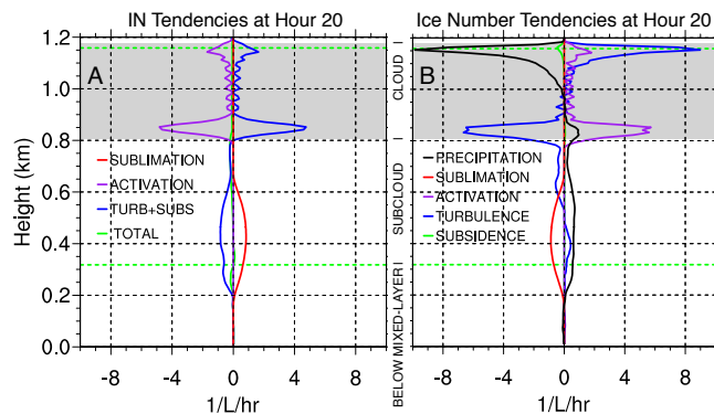
Figure 6. (a) N_{\text{IN}} and (b) N_{\text{ICE}} averaged over 0.5 h at hour 20, in units of \text{L}^{-1} \text{ h}^{-1} . Gray shading indicates the extent of the cloud layer. Green dash lines indicate the top and bottom of the mixed layer.
