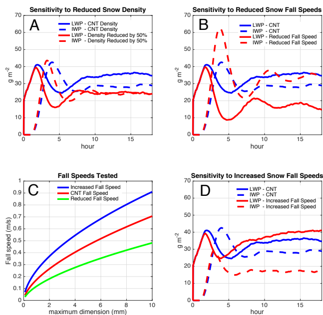
Figure 4. (a, b, d) Sensitivity of LWP and IWP to snow density and fall speeds. LWP shown with solid lines and IWP shown with dashed lines, in units of \text{g m}^{-2} . (c) Fall speeds used in sensitivity studies, in units of \text{m s}^{-1} . (a) Sensitivity to reducing snow density from 100 to 50 \text{ kg m}^{-3} (red lines) using Control (CNT) fall speeds (red line in c). (b) Sensitivity to reducing snow fall speeds (green line in c) using Control snow density (red lines). (d) Sensitivity to increasing snow fall speeds (blue line in c) using Control snow density (red lines).
