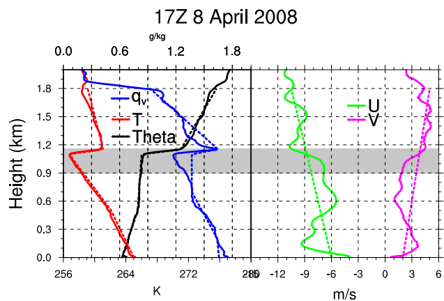
Figure 1. Sounding measured at 17:34 UTC 8 April 2008 at Barrow, Alaska ( 71.338^{\circ} N, 156.68^{\circ} W). Left: water vapor mixing ratio ( q_v ), temperature ( T ), and potential temperature ( \theta ), in units of \text{g kg}^{-1} , kelvin, and kelvin respectively. Right: zonal wind ( U ) and meridional wind ( V ), in units of \text{m s}^{-1} . Gray shading marks the extent of the cloud layer. The dashed lines show the initial profiles used in the WRFLES experiments. The dashed line overlying water vapor mixing ratio is the initial profile for the total water mixing ratio.
