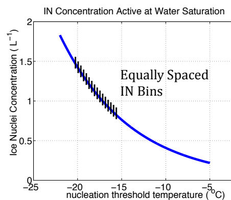
Figure 2. IN number concentration active at water saturation vs. temperature based on the empirical relationship derived in DeMott et al. (2010; blue line) used to initialize IN number concentration in each bin. Black vertical lines indicate threshold temperatures for nucleation in the 16 IN bins. Note that additional IN become available for nucleation at colder temperatures, such that, for example, at -20.2 °C (the coldest temperature in the Control simulation) the total number of IN available for activation is \sim 1.5 \text{ L}^{-1} .
