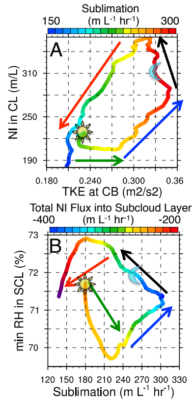
Figure 12. (a) Phase diagram of TKE at cloud base vs. N_{\text{ICE}} in the cloud layer starting at peak shortwave hour 40, in units of \text{mL}^{-1} and \text{mL}^{-1} \text{h}^{-1} , respectively. Colors show sublimation in units of \text{mL}^{-1} \text{h}^{-1} . (b) 24 h phase diagrams of sublimation vs. minimum relative humidity in the subcloud layer starting at peak shortwave hour 40, in units of \text{mL}^{-1} \text{h}^{-1} and %, respectively. Colors show total N_{\text{ICE}} flux at cloud base, \text{mL}^{-1} \text{h}^{-1} . Hours 42–47, 47–50, 50–56, and 57–62 indicated with green, blue, black, red arrows, respectively. Minimum shortwave indicated with the moon symbol. Maximum shortwave indicated with the sun symbol.
