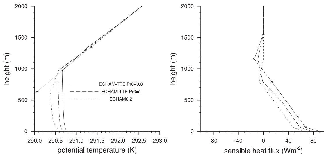
Figure 3. (left) Potential temperature and (right) sensible heat flux profiles for an idealized dry convective boundary-layer case with prescribed surface heating ( u_{geo} = 10 \text{ ms}^{-1} ) averaged over 1 h after 6 h of model integration. Results are from the single-column model using ECHAM6.2 and ECHAM-TTE, using neutral limit Prandtl numbers of 1 and 0.8 in ECHAM-TTE.
