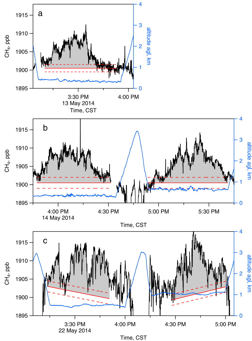
Figure 4. Time series of CH 4 measurements (black) from the five transects downwind of the Bakken shale region shown in Figure 3. The blue trace shows the Twin Otter altitude above ground level. The red trace represents the background CH 4 used for the flux calculations; the dashed red traces represent the estimated \pm 1\sigma uncertainty of the background. The shaded areas show the CH 4 enhancement above the background along the transects.
