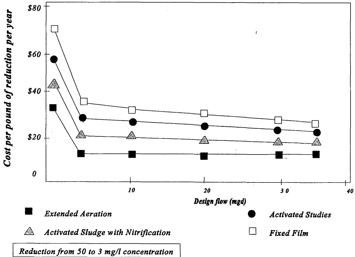
FIGURE 4.8. Planning-level biological nitrogen removal retrofit cost curves.
