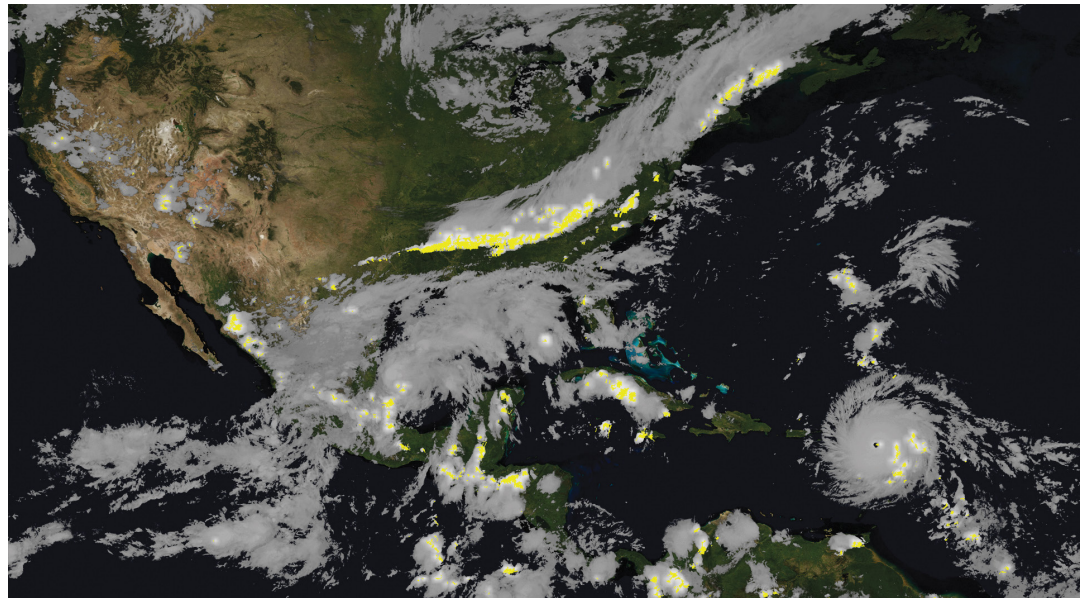
Figure 1. Depiction of clouds and lightning as viewed by the GOES-16 Advanced Baseline Imager (ABI) and Geostationary Lightning Mapper (GLM) during Hurricane Irma (2017).
