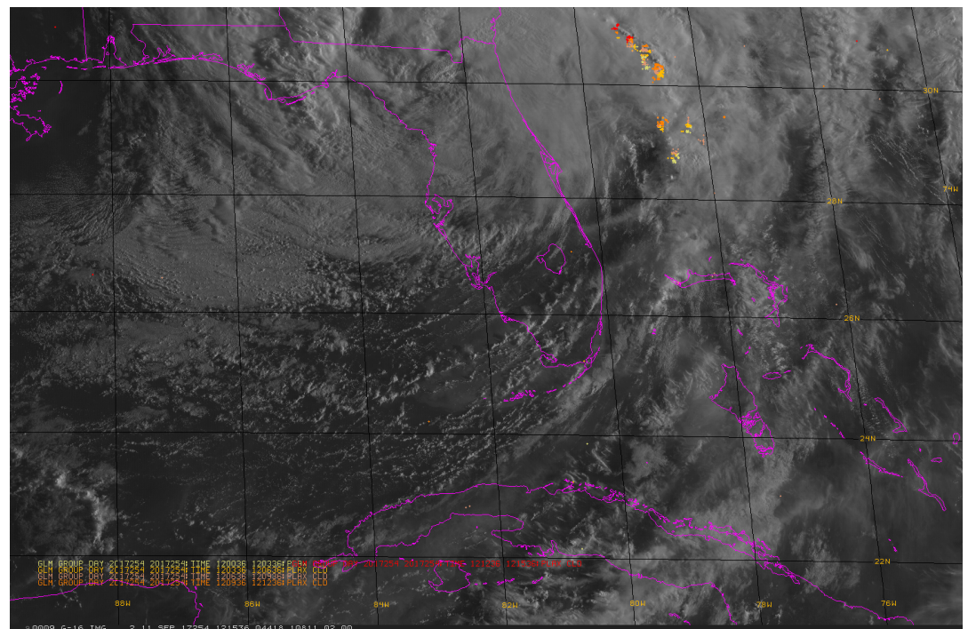
Figure 1. Groups of GOES-16/GLM observations during tropical cyclone Irma (2016) (Courtesy: University of Wisconsin/CIMSS and Colorado State University/CIRA).
