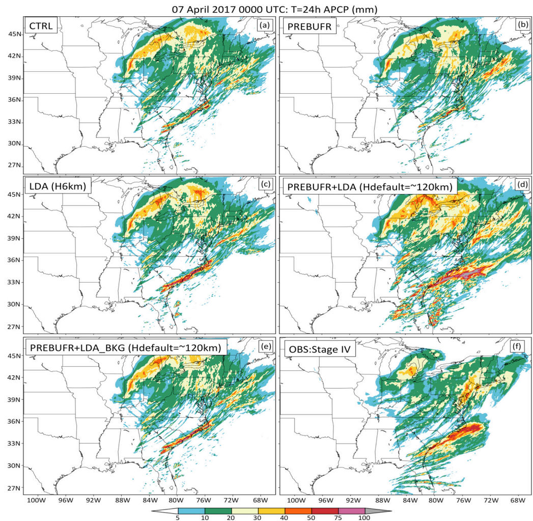
Figure 2. As in Figure 1 but for the simulated 24-h accumulated precipitation (APCP). For reference, the observed (Stage IV) 24-h APCP fields are shown in (f).
