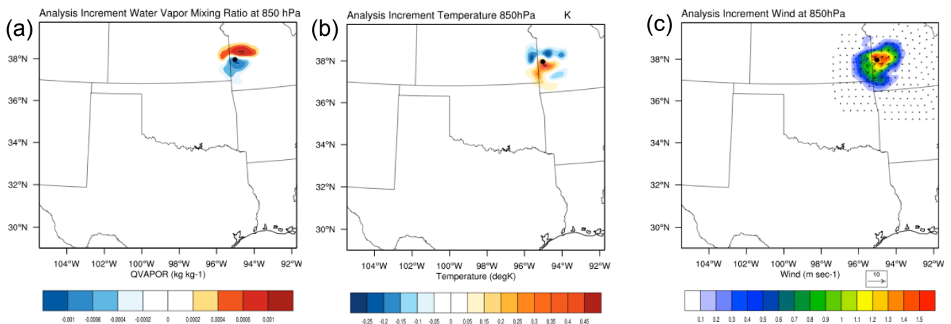
Figure 4. Analysis increments of (a) water vapor mixing ratio ( \text{kg kg}^{-1} ), (b) temperature ( \text{degK} ) and (c) wind ( \text{m sec}^{-1} ) at 850 hPa. The black dot shows the location of a single lightning observation ( 37^\circ\text{N} , 95^\circ\text{W} ). Dipoles of positive and negative analysis increments can be observed at either end of the single observation in the specific humidity and temperature plots but with opposite signs. 850 hPa winds show a positive analysis increment with maximum values coinciding with the region of positive temperature increment, and anti-cyclonic circulation can be observed around the location of the single observation. These increments are a clear indication of the information content a single lightning strike can spread horizontally into the analysis.
