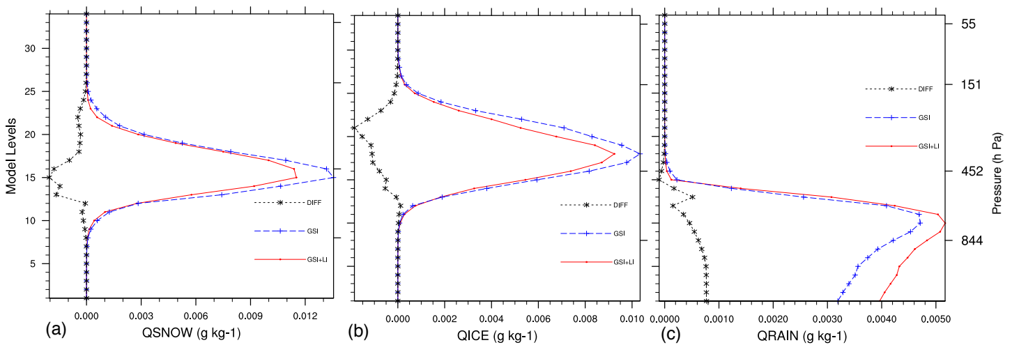
Figure 5. Valid at 26 AUG 2013 0600 UTC. The blue curve represents the control experiment with the assimilation of conventional observations, only (GSI). The red curve represents the assimilation of lightning and conventional observations (GSI+LI). The black curve shows the difference between both experiments. Note that in (a) and (b) the assimilation of lightning (red) lead to decreases in the concentration of ice and snow mixing ratios, while increasing rain mixing ratio (red) in (c).
