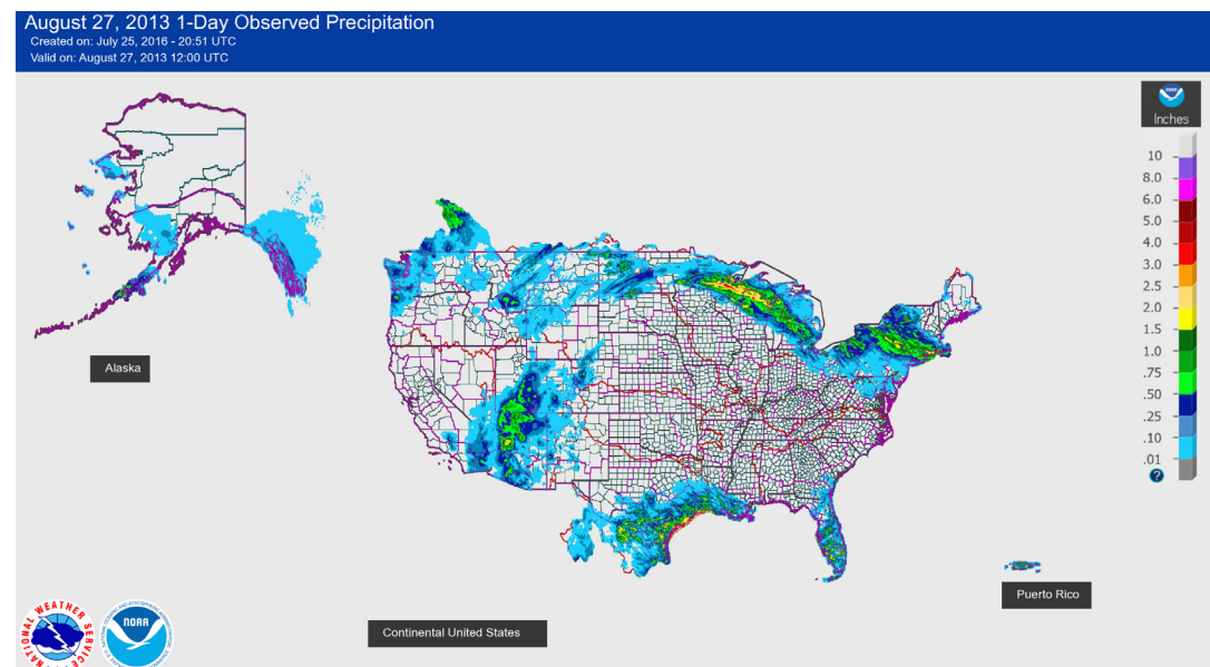
Figure 3. 24-hr precipitation valid at 2013-08-27_12:00:00 (Courtesy: NWS). Note the region of maximum precipitation near the Arizona-Nevada border, which coincides with the region of a positive analysis increment in specific humidity shown in Fig. 2. The assimilation of lightning observations has a positive impact in the initial conditions of the GFS model.
