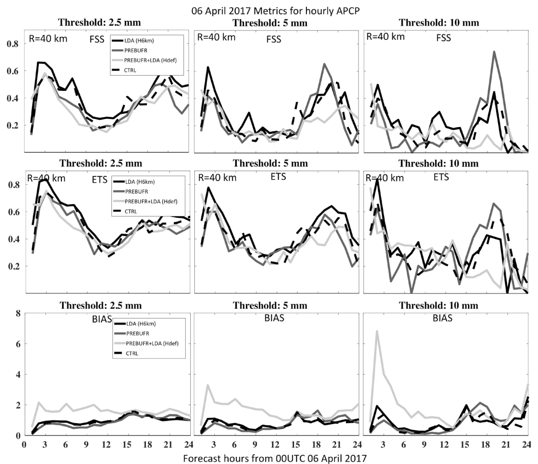
Figure 3. Domain wide fractions skill score, equitable threat score, and frequency bias for various simulated APCP thresholds for LDA (H6km), PREBUFR, PREBUFR+LDA (Hdefault) and the control run (CTRL).
