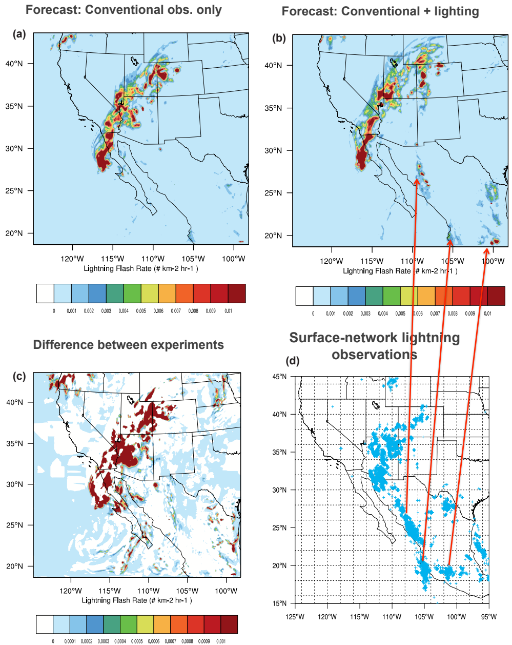
Figure 6. A 3-hour forecast of lightning flash rate (strikes per km 2 per hour) valid at 25 AUG 2013 1200 UTC: (a) after assimilating conventional observations only, (b) after assimilating conventional and lightning observations, (c) the difference between both experiments, and (d) raw WLLN lightning observations.
