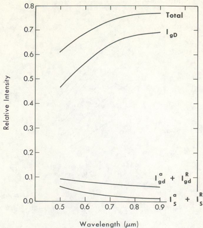
Figure 14.--Components of the relative intensity outward from the nadir direction at the top of a turbid atmosphere over White Sands for a solar zenith angle \theta_0 = 0^\circ
