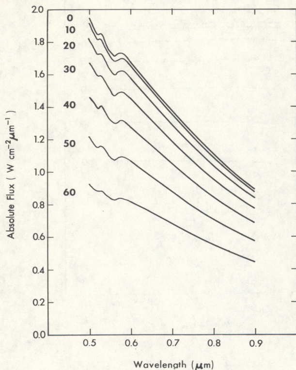
Fig. 7.--Total spectral flux of radiation incident at the surface of White Sands for a Rayleigh atmosphere and various zenith angles of the sun.
