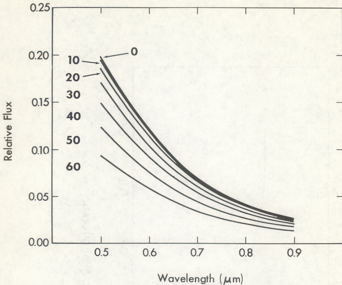
Figure 4.--Relative flux F_{D_S} + F_{d_s} + F_{D_S}' downward at the surface of White Sands for a Rayleigh atmosphere and various solar zenith angles.
