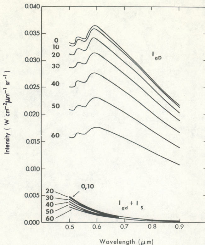
Figure 8.--Intensity I_{gD} and I_{gd} + I_s of solar radiation directed outward from the nadir direction at the top of a Rayleigh atmosphere over White Sands.
