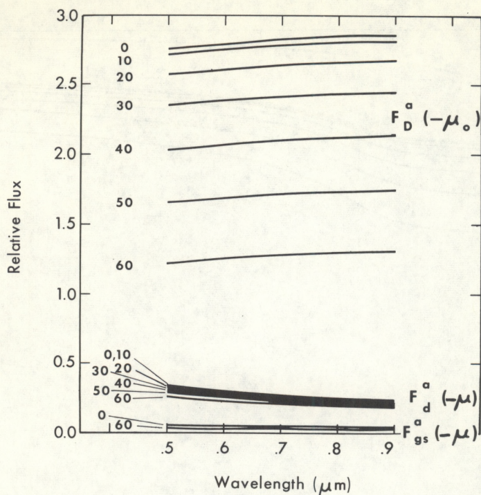
Figure 12.--Relative flux of the various components of solar radiation downward at White Sands for an aerosol atmosphere and various solar zenith angles.
