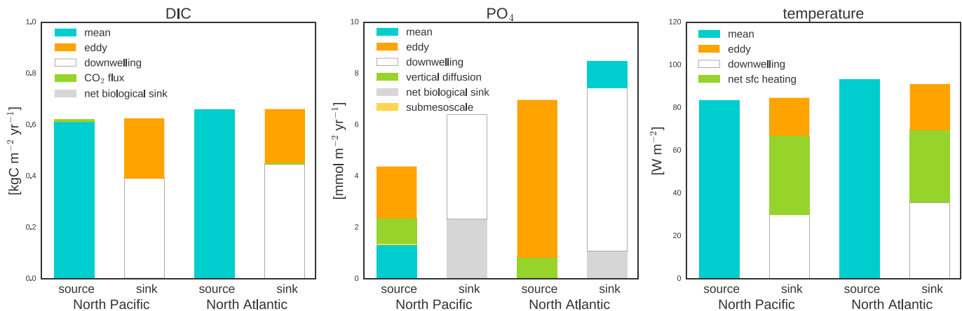
Figure 8. Annual mean DIC (left), PO 4 (middle), and temperature (right) budgets for the North Pacific and North Atlantic subtropical gyres. Mean (cyan) corresponds to the mean horizontal advective transport of each tracer, eddy (orange) the eddy horizontal advective transport, and downwelling (white) the transport across the isopycnal at the base of the ventilated pycnocline, computed as the residual between the 3-D advective convergence within the gyre bowl and the total cross-boundary horizontal transport. CO 2 flux (green on the left panel) is the air-sea CO 2 flux, net biological sink (gray on the left panel) is the biological consumption and remineralization of DIC, vertical diffusion (green on the middle panel) is the flux of PO 4 across the bottom of the layer via parameterized vertical mixing, net biological sink (gray on the middle panel) corresponds to the net biological consumption of PO 4 integrated over the vertical layer, submesoscale (yellow on the middle panel) is the PO 4 supply due to the parameterization of submesoscale mixed layer instabilities, and net sfc heating (green on the right panel) is the net surface heating including the effect of longwave and shortwave penetrating radiation, as well as sensible and latent heat fluxes. Additional terms, including vertical diffusion and submesoscale transport of DIC and temperature, are all at least 3 orders of magnitude smaller than the shown terms and therefore excluded from the figure. Note that the imbalance between the source and sink, particularly evident for PO 4 , is due to the non-negligible tendency term, amounting to -2.3 mmol/m 2 /year for the North Pacific and -1.5 mmol/m 2 /year for the North Atlantic subtropical PO 4 budgets. This imbalance is associated with a time tendency in the model over the 10-year period we analyzed. DIC = dissolved inorganic carbon.
