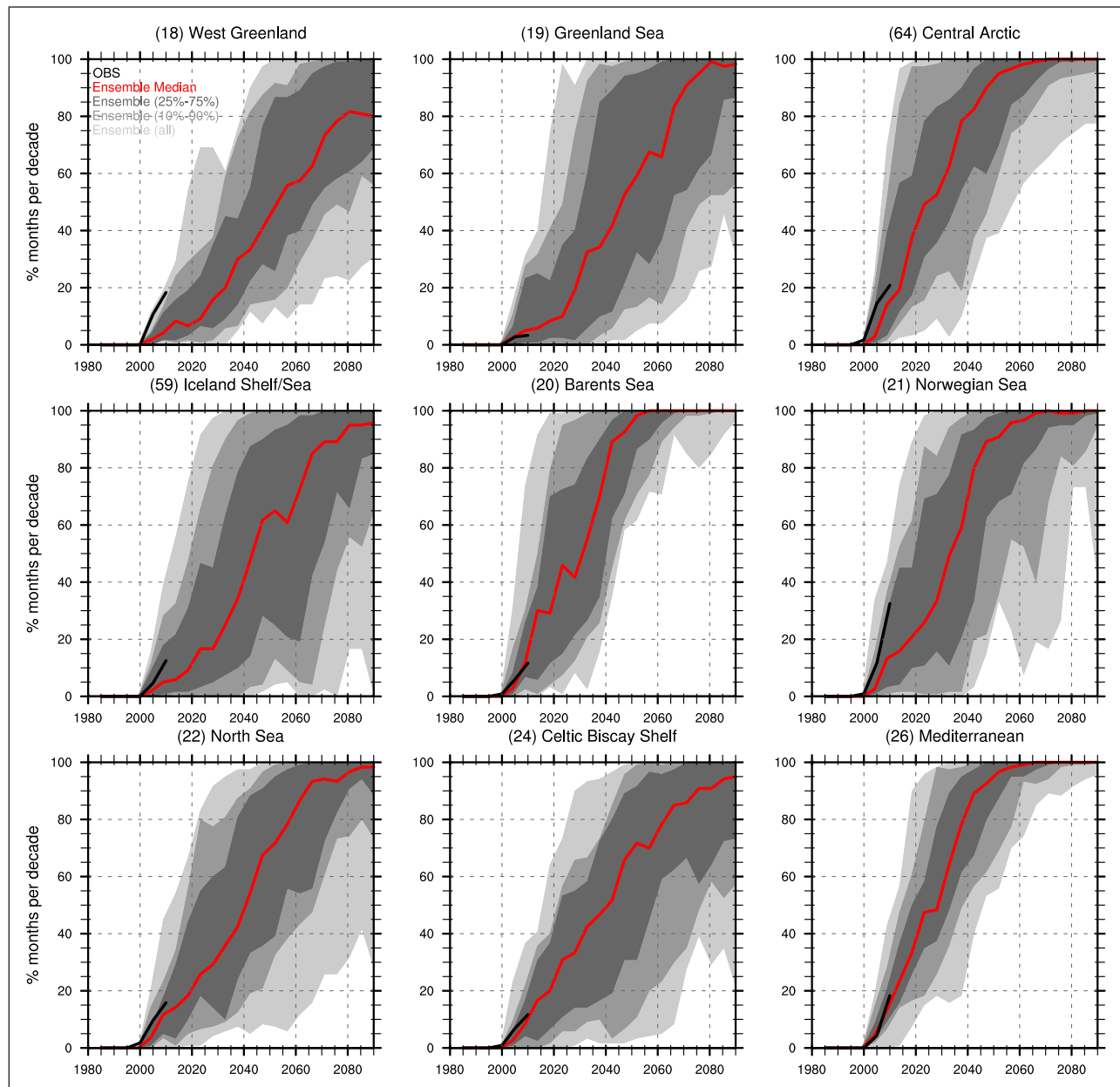
Figure 14: Percent of monthly SST anomalies in each decade that exceed the monthly maximum during 1976–2005. Results are shown for CMIP5 models in the LMEs in the Arctic and around Europe. The ensemble median is red and Hadley SST observations are black. The outer envelope (light gray) shows the ensemble max/min range. The 2 nd envelope (medium gray) shows the 10 th –90 th percentile range of the ensemble and the inner envelope (dark gray) indicates the inter-quartile range (25 th –75 th percentile). The decades were sampled every five years in overlapping 10-year periods for smoothness. By mid-century most regions exceed the maximum during the historical period (1976–2005) more than 80% of the time. DOI: https://doi.org/10.1525/elementa.191.f14
