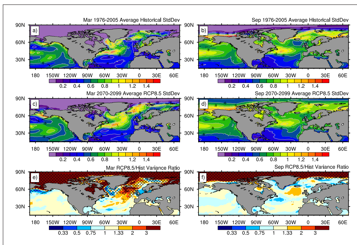
Figure 9: CMIP5 ensemble mean interannual SST standard deviation (°C). The year-to-year SST standard deviation ( \sigma ) for the historical period 1976–2005 (a, b) and the future period 2070–2099 (c, d), along with the future/historical SST variance ( \sigma^2 ) ratios (e, f), for both March (a, c, e) and September (b, d, f). The SST anomalies are computed for each model separately, de-trended within their respective periods, and the standard deviation (and the variance) are computed for each individual model and then averaged together. The variance ratios are cross-hatched, where >50% of the models show a significant change at the 95% level. Significant changes in SST variance are mainly found at higher latitudes and in the northern north Atlantic in winter. DOI: https://doi.org/10.1525/elementa.191.f9
