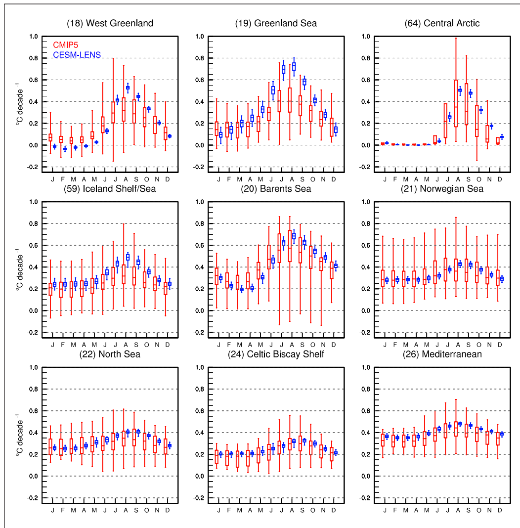
Figure 4: SST trends during the period 1976–2099 from LMEs in the Arctic and around Europe. SST Trends ( ^{\circ}\text{C decade}^{-1} ), computed for each model from the CMIP5 (red) and CESM-LENS (blue) experiments, are shown in box and whiskers format, where the end points indicate the maximum and minimum values, the box boundaries indicate the inter-quartile range (25% to 75%), and the median is the central line. The larger spread in CMIP5 relative to CESM-LENS indicates the range of trends is substantially greater among different models than due to internal variability in an individual model. DOI: https://doi.org/10.1525/elementa.191.f4
