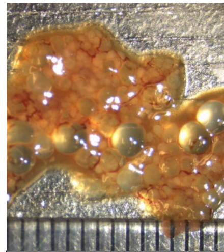
Figure 4. Image showing the hydrated eggs from an opah.
