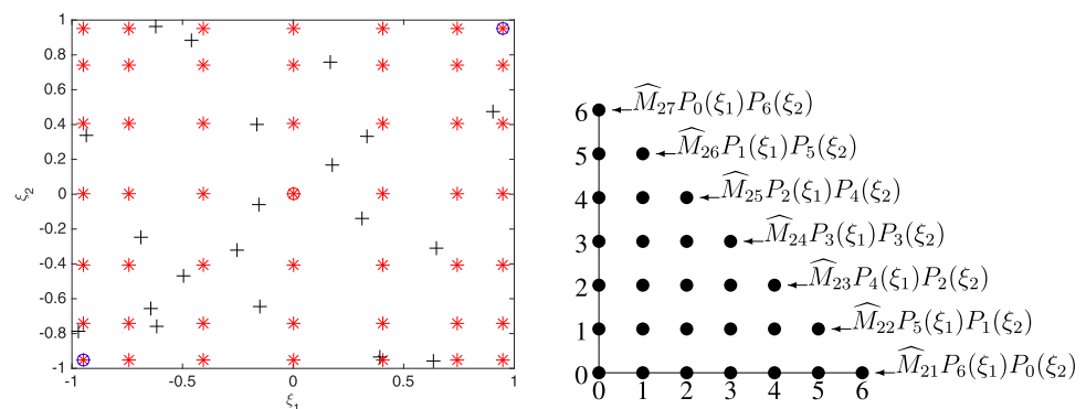
Figure 3. (left) Gauss Legendre quadrature (sample) points in the uncertain \xi_1 - \xi_2 space (red *); the center red circle shows to unperturbed run, while the blue circles correspond to the largest negative and positive perturbations; the black (+) signs show the settings of the 20 independent validation runs. (right) the polynomial degree in \xi_1 and \xi_2 retained in the series.
