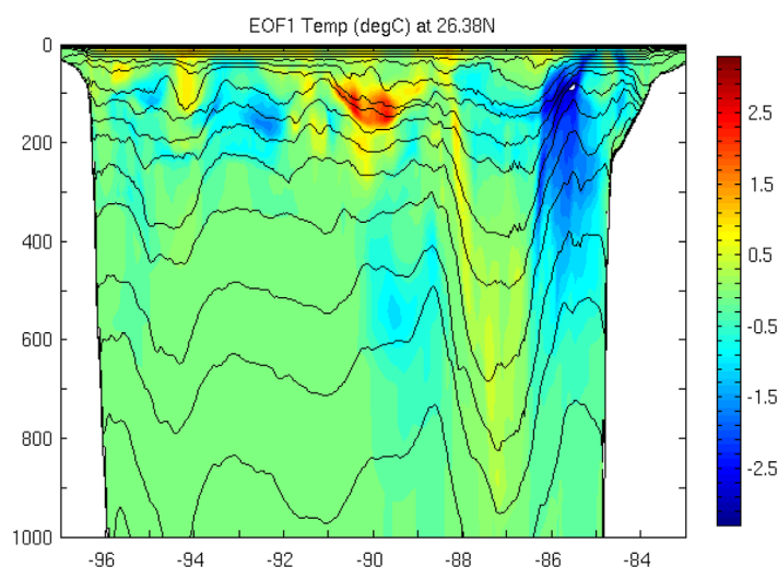
Figure 2. Vertical slice along 26.4N showing the temperature perturbations 1 day after the start of the simulation. The first mode shows a strong 2.5°C cooling in the vicinity of the frontal cyclones. The warm perturbation around 90W is at the southern edge of a small anticyclone NW of the LC.
