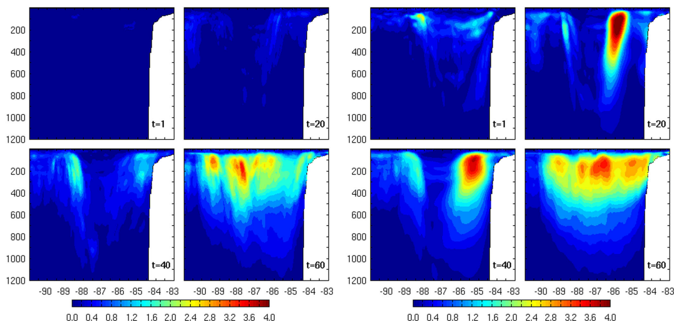
Figure 9. (left) The evolution of the PC-error associated with the temperature field along 25°N; the errors build up gradually with time and exceed 3°C by day 60 in the 200–400 m depth range. (right) The evolution of the temperature standard deviation with the uncertainty manifesting itself primarily on the eastern side of the loop current. On day 60 the PC-error is about 100% of standard deviation.
