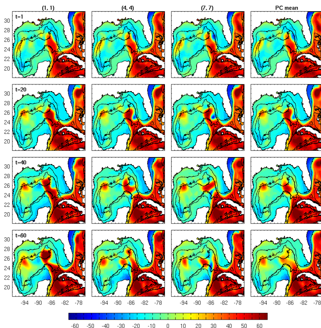
Figure 4. Time evolution of SSH realization (1,1) (first column) with weakest frontal eddy; of unperturbed realization (4,4) (second column) revealing a medium strength frontal eddy; and realization (7,7) (third column) with strongest frontal eddy. The fourth column shows the PC-ensemble mean of all 49 realizations, aka the 0-th mode of the PC-series. The times shown are in days since the start of the simulation, and SSH units are in cm.
