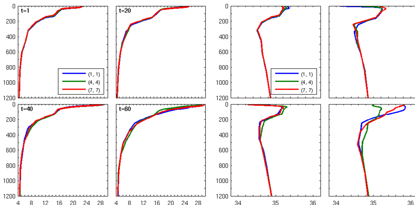
Figure 7. (left) Temperature and (right) salinity profiles at the DWH for the reference and extreme perturbations.
