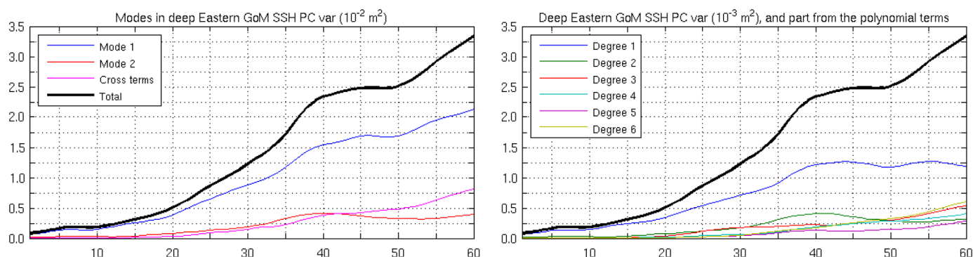
Figure 12. (left) Evolution of the SSH variance over the Deep Eastern part of the GoM (east of 90W and deeper than 2000 m) as contributed by the two modal perturbations and their interaction. (right) Contribution to the SSH variance over the deep Eastern GoM by the different polynomial orders. The thick black lines shows the total variance whereas the thin black lines shows the contribution to the variance injected by the different polynomial orders.
