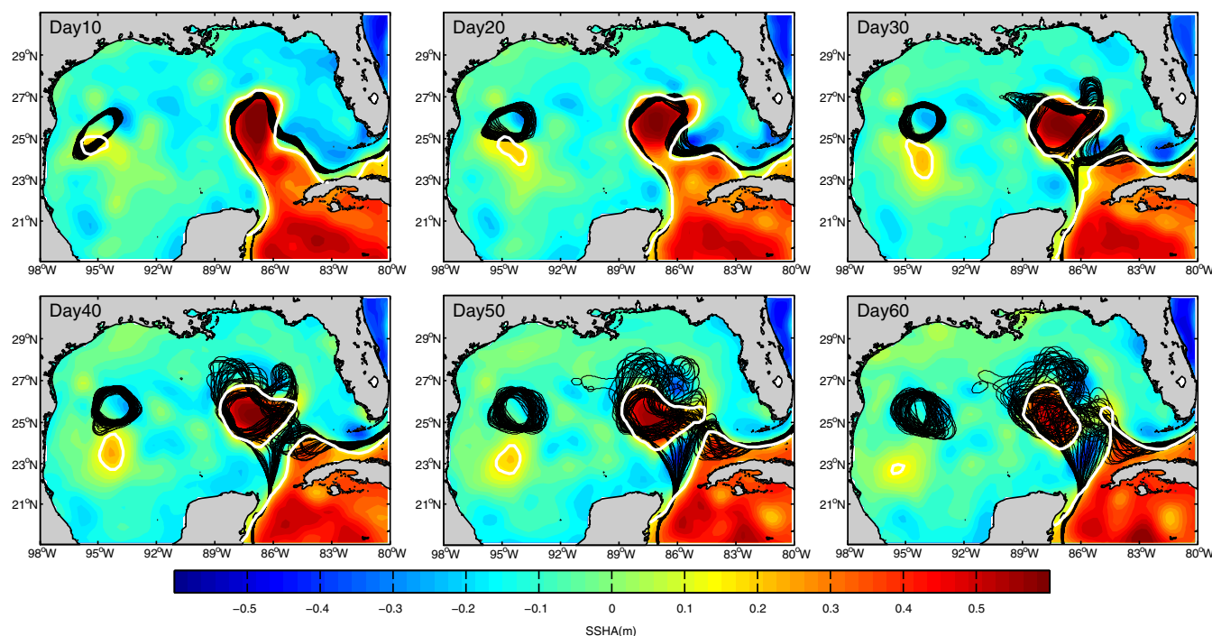
Figure 6. Time evolution of the SSH anomaly from AVISO altimetry data (color), with the Loop current edge, as defined by the 17 cm contour, in the PC ensemble (black lines) and in the AVISO data (white line).
