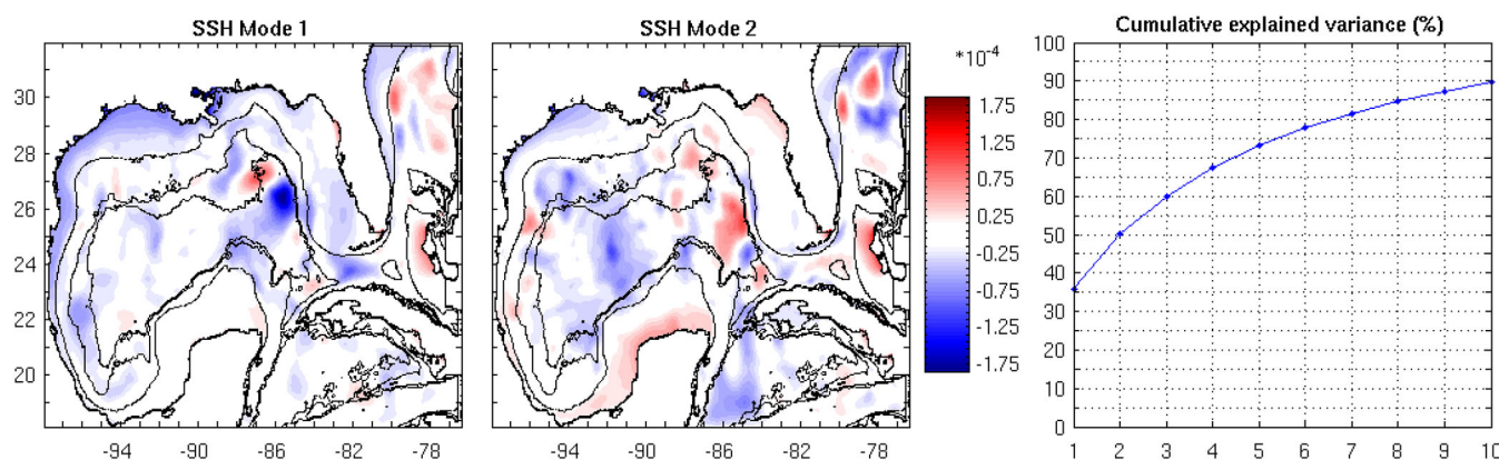
Figure 1. SSH patterns for mode 1 and 2 perturbations (left and middle) along with the cumulative variance explained by the first 10 modes.
