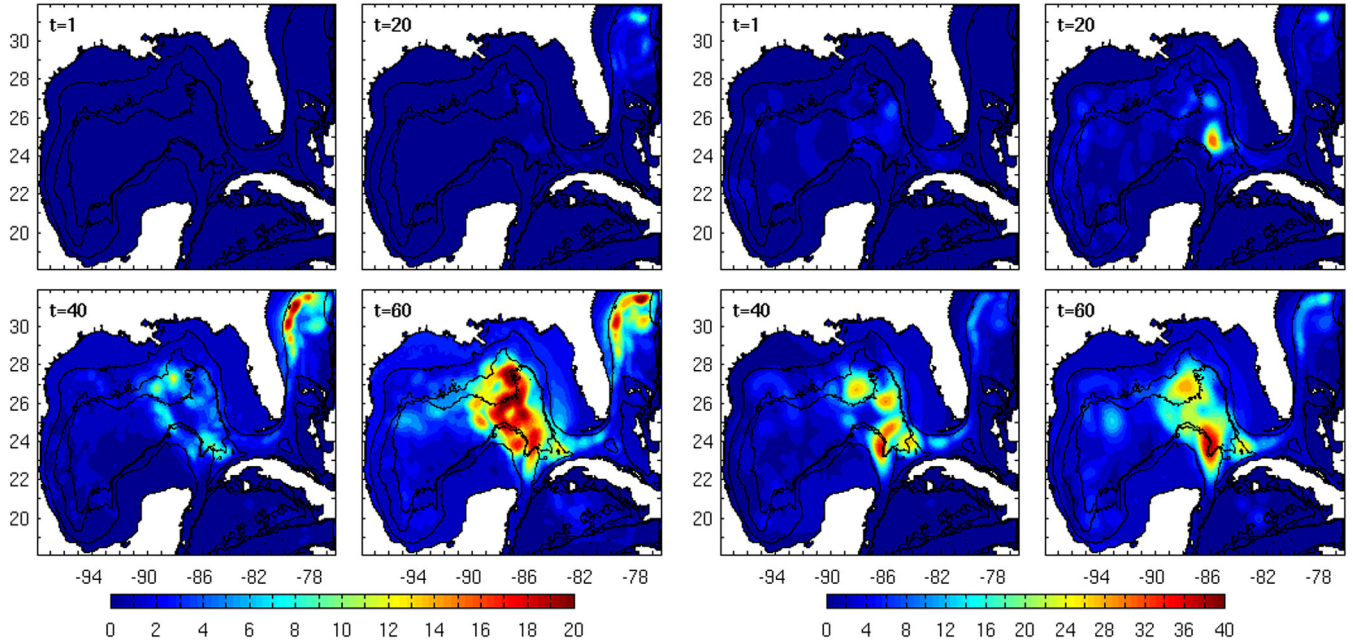
Figure 8. (left) Temporal evolution and spatial distribution of the PC error, \|\epsilon\| (shown in cm), associated with SSH. The errors grow in time with their maxima located primarily in the dynamically active LC region. (right) Evolution of SSH stddev (in cm) as estimated from the PC-series; the areas of largest uncertainties are located in the LC region.
