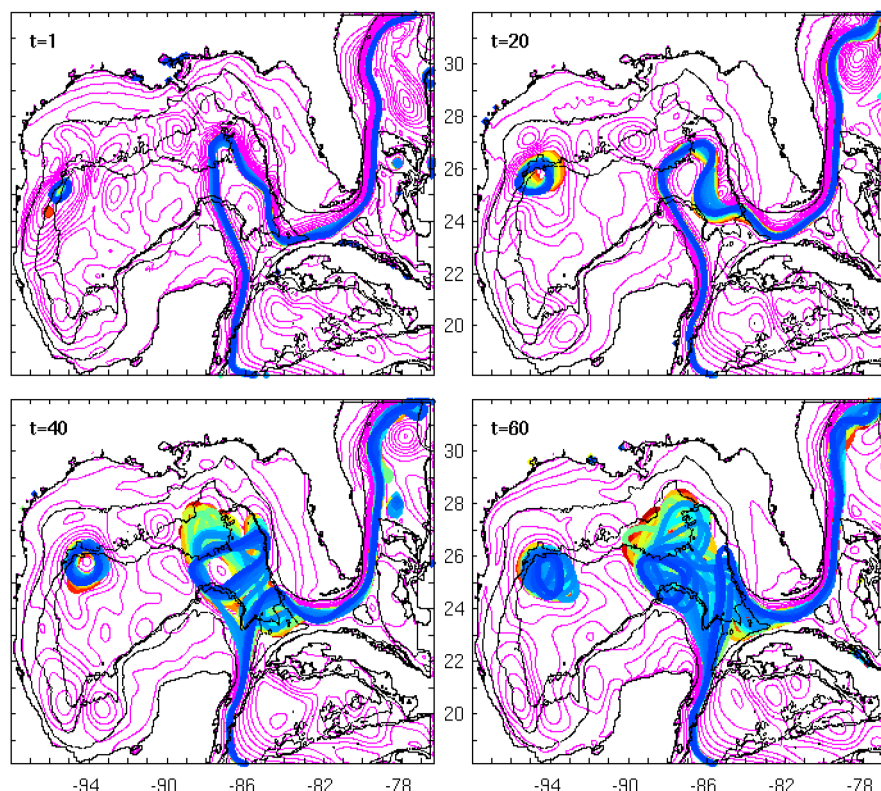
Figure 5. Loop Current evolution for all realizations. The thin magenta contours are the PC-mean of the SSH field, while the thick lines indicate the LC edge as defined by the 17 cm contour. The bluish thick lines are associated with the strong frontal eddy realizations whereas the reddish ones are associated with the weak frontal eddy.
