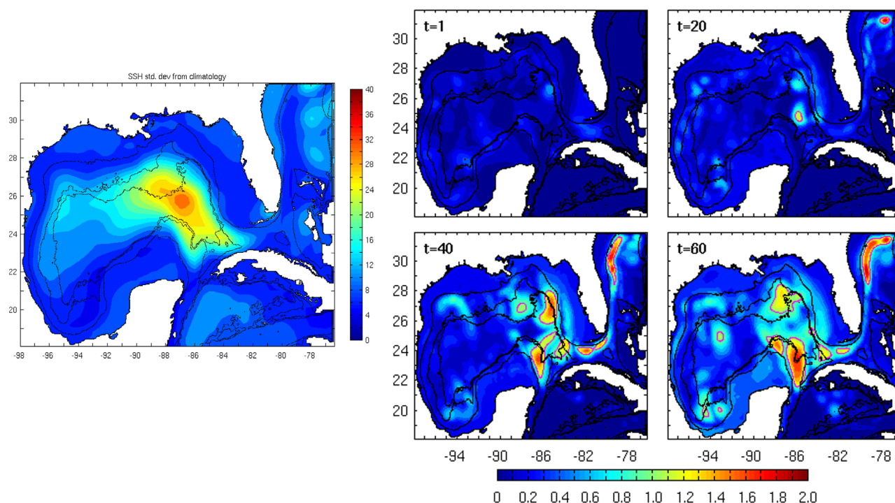
Figure 10. Variance Ratios: (left) The climatological SSH standard deviation as inferred from AVISO. (right) The evolution of the spatial distribution of the ratio of the forecast standard deviation to climatology standard deviation for SSH (from AVISO).
