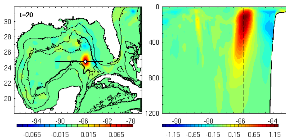
Figure 11. Covariances between one value of SSH (white dot circled in black) and the GOM SSH, and between the same SSH value and the vertical temperature along the longitude line indicated on the left figure. The SSH point location is marked on the section with dashed line. The units are m^2 and m^\circ C .
