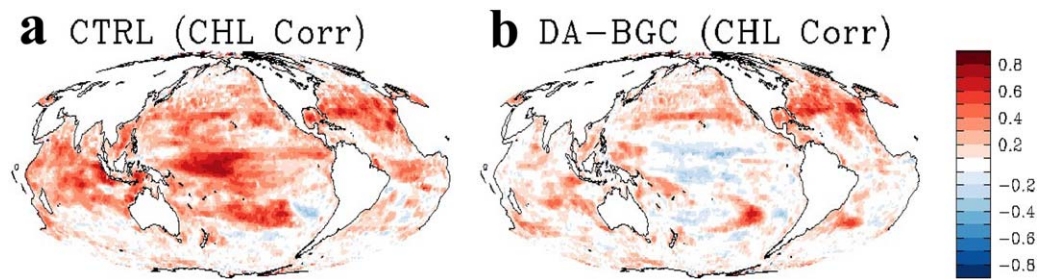
Figure 3. Temporal correlation maps of simulated chlorophyll from (a) CTRL and (b) DA-BGC with satellite-retrieved chlorophyll concentrations. The correlation coefficients are calculated after removing monthly climatology during the analyzed period September 1997 to December 2015. The satellite chlorophyll data are bilinearly interpolated onto the regular 1.0^\circ \times 1.0^\circ model grid before calculating correlation coefficient.
