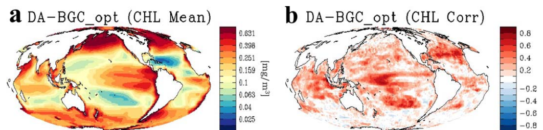
Figure 9. (a) Annual mean surface chlorophyll simulated from DA-BGC_opt. (b) Correlation map of chlorophyll between DA-BGC_opt and satellite data.
