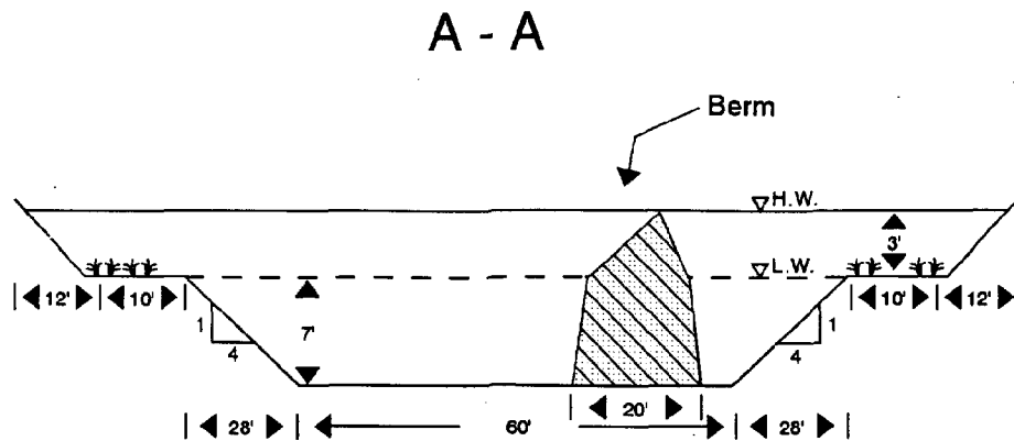
Figure 7-10. Cross-sections of Stormwater Management Lake
