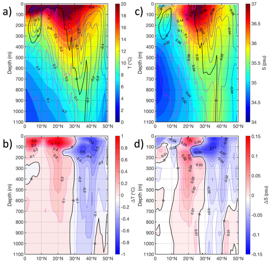
FIG. 10. The JAMSTEC time-mean profiles of (a) temperature and (c) salinity (color) averaged between 10° and 40°W, with the meridional gradients (contours) of temperature [ ^{\circ}\text{C} (100 \text{ km})^{-1} ] and salinity [ \text{psu} (100 \text{ km})^{-1} ] gradients, respectively. The differences of the low-pass filtered (b) temperature and (d) salinity profiles between October 2010 (high sea level near the eastern boundary) and October 2008 (low sea level near the eastern boundary).
