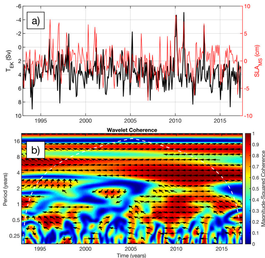
FIG. 4. (a) The monthly time series of SLA MS from satellite altimetry and T_{EK} at 26.5°N computed from the ERA-Interim zonal wind stress and (b) the wavelet coherence between the time series in (a). Note that the y axis for T_{EK} is reversed. The direction of the arrows in the coherence plot corresponds to the phase lag on the unit circle, with the backward direction indicating an out-of-phase relationship. The cone of influence in the coherence plot (white-dashed curve) indicates where edge effects occur in the coherence data.
