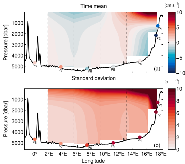
Figure 4. (a) Time-mean and (b) standard deviation of the absolute meridional geostrophic velocity (cm/s) determined between pairs of Current and Pressure recording Inverted Echo Sounders (CPIES). The colored dots represent the mean and the standard deviation of the direct measurement of velocity from the bottom current meters at the CPIES positions, respectively. Black vertical dotted lines denote the positions of the estimated geostrophic velocity profiles at the midpoints between CPIES.
