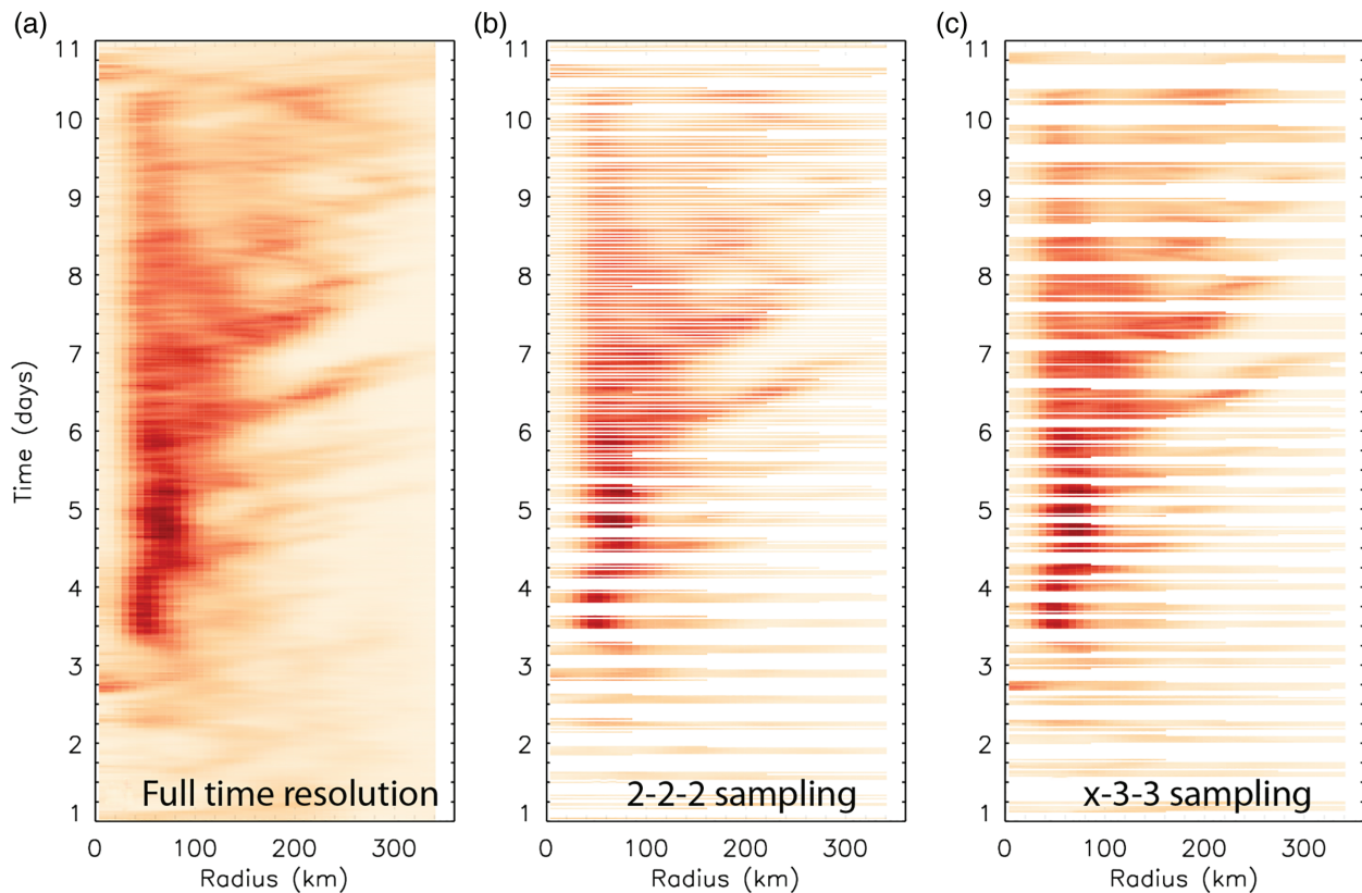
FIGURE 2 Hovmöller diagrams showing precipitation intensity as a function of time and radial distance from the centre of the storm for the WRF Hurricane Nature Run. (a) shows the continuous evolution of precipitation. (b) shows the temporal sampling as observed from the baseline 2-2-2 orbital configuration. (c) shows the temporal sampling as observed from a 3-3 orbital configuration
