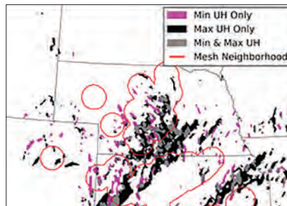
FIGURE 10 (left). Spatial Contribution of 2–5 km AGL Minimum (magenta), Maximum (black), and Full (gray) 24-h UH to Severe ( \geq 29 mm) Hail MESH 40 km Neighborhoods (red circles). Data from 0000-UTC initialized NSSL-WRF on 08 May 2016. Image credit: Provided by Israel Jirak.
