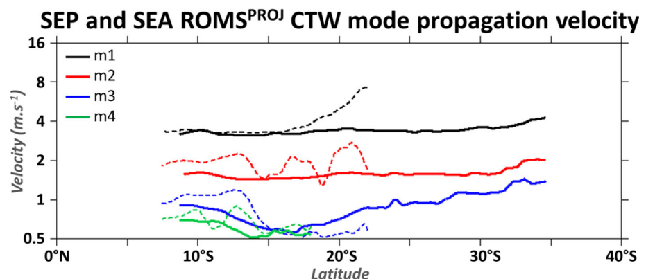
Figure 9. Similar to Figure 4, but CTW mode propagation velocity (m.s -1 ) are estimated from ROMS PROJ CTW modes amplitude. For each CTW mode and each latitude, propagation velocity is estimated by linear regression that best fits the maximum lagged correlation analysis within a 5° latitudinal window (similar to Figure 8).
