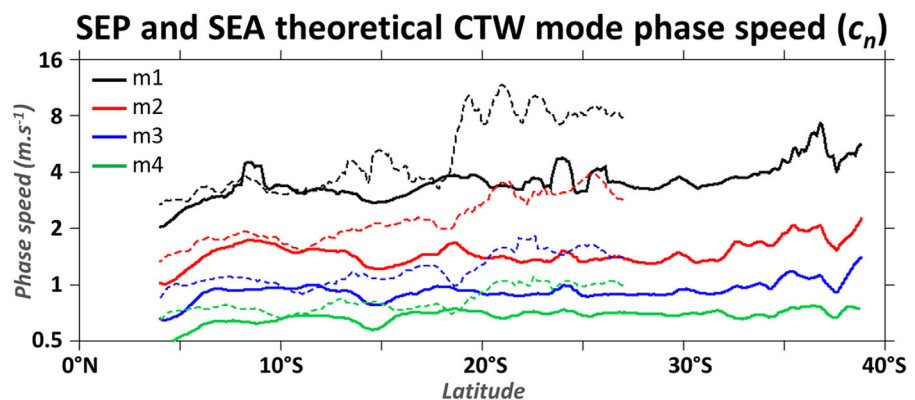
Figure 4. CTW theoretical phase speed (eigenvalues obtained from the CTW decomposition) in function of latitude along the coasts of the SEP (plain lines) and the SEA (dashed lines). CTW mode 1, 2, 3, and 4 are in black, red, blue, and green, respectively. Unit is \text{m.s}^{-1} . To better visualize fast and slower phase speed, we use a Log2 vertical scale.
