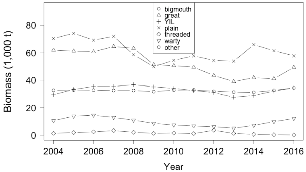
Figure 10. Random effect estimates of the six most common sculpin species in the BSAI, in 1,000 t.
