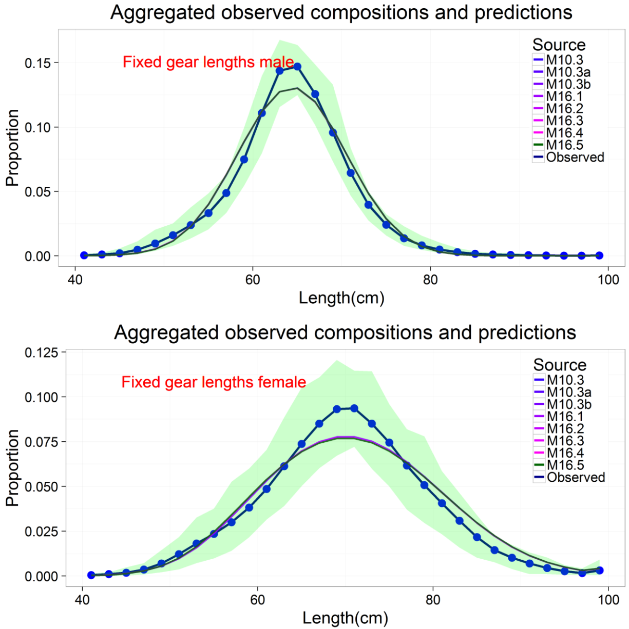
Figure 3.31. Domestic fixed gear fishery length compositions aggregated across years and with average fits from the 8 model options. Mean observed are the blue dots, the green bands are the 90% empirical confidence intervals.
