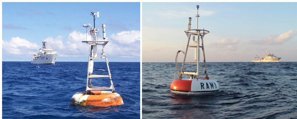
Figure 2. Buoy, tower, and meteorological sensors for ATLAS (left) and T-Flex (right) moorings.
