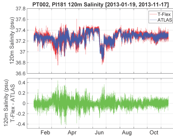
Figure 17. Test 4 10-min salinity (PSU) from 120 m T-Flex PT002 (blue) and ATLAS PI181 (red) sensors and difference (green).
