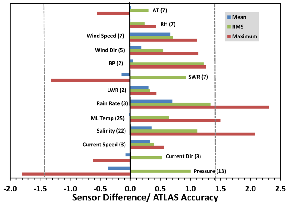
Figure 19. Ratio of mean, RMS, and maximum difference of T-Flex and ATLAS sensors divided by the expected ATLAS accuracy. The number of sensor pairs for each sensor type is indicated in parentheses. The RMS and maximum were computed from each test mean difference. Vertical dashed lines indicate the expected standard deviation for normalized ATLAS minus T-Flex mean differences assuming that sensors for the two mooring systems have comparable accuracy and that errors are normally distributed.
