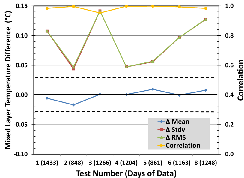
Figure 15. Mean (blue), standard deviation (red), and RMS (green) difference and correlation coefficients ( R^2 , yellow) between T-Flex and ATLAS daily mixed layer temperature. Dashed lines indicate expected accuracy of the ATLAS sensors. The numbers of daily mean values per test are in parentheses on the x axis.
