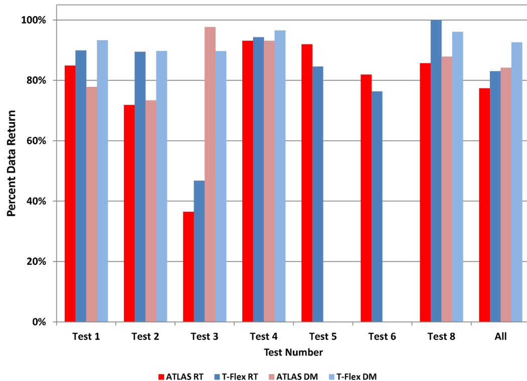
Figure 3. Real time (RT) and delayed mode (DM) data return averaged over all sensors for each of seven tests and for all tests combined.
