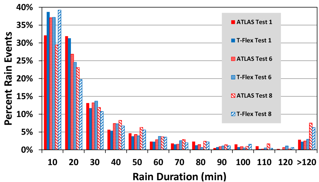
Figure 11. Percentage distribution of rain events by duration (min). Percentages are relative to the total number of rain events composed of continuous rain rates above 0.4 mm hr -1 . ATLAS data are in red and T-Flex data in blue.
