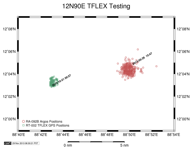
Figure C1. Mooring locations reported by Argos (ATLAS RA092) and GPS (T-Flex RT002).
