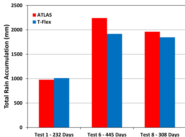
Figure 13. ATLAS (red) and T-Flex (blue) total rain accumulation for Tests 1, 6, and 8.
