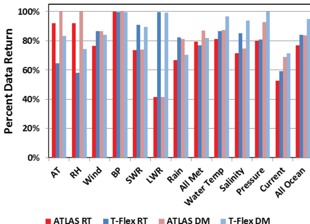
Figure 4. Real time (RT) and delayed mode (DM) data return averaged by sensor type for all tests combined.
