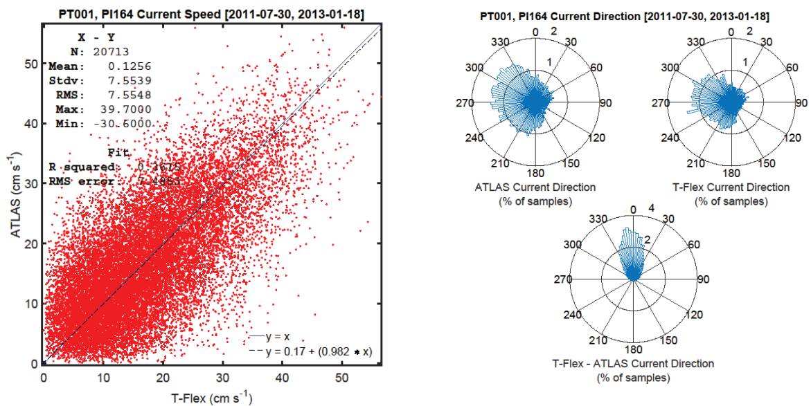
Figure 18. Test 2 current speed scatter plot (left) and current direction histogram (right) for T-Flex PT001 and ATLAS PI164.
