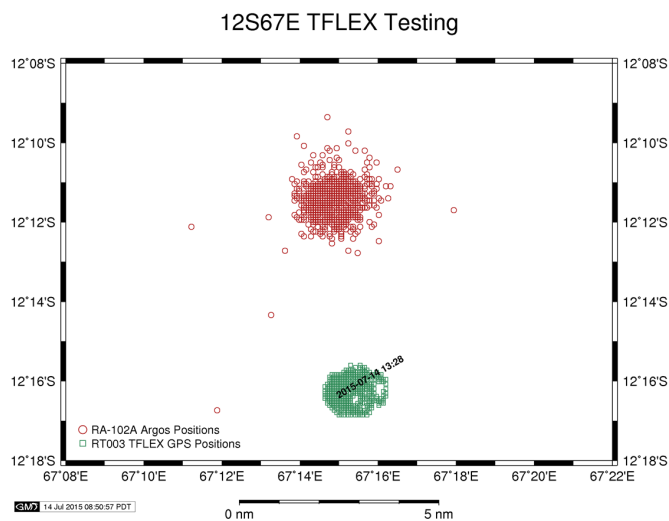
Figure E1. Mooring locations reported by Argos (ATLAS RA102) and GPS (T-Flex RT003).
