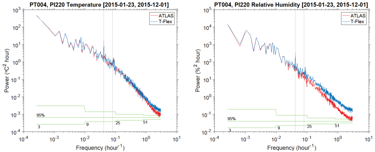
Figure 6. Left: Test 8 air temperature spectra from T-Flex PT004 (blue) and ATLAS PI220 (red) sensors. Right: Test 8 relative humidity spectra from T-Flex PT004 (blue) and ATLAS PI220 (red) sensors. Green lines indicate 95% confidence limits, with numbers below giving the number of raw periodogram points averaged for a given frequency band.
