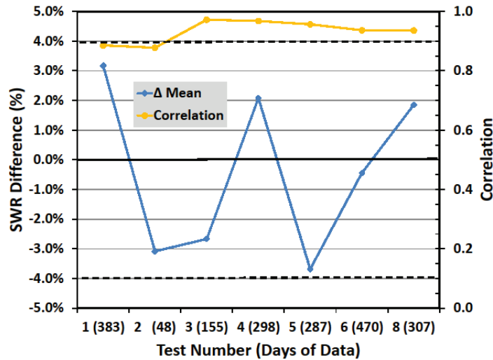
Figure 8. Mean (blue) and correlation coefficients ( R^2 , yellow) between T-Flex and ATLAS daily mean short-wave radiation time series. Dashed lines indicate expected accuracy of the ATLAS sensors. The numbers of daily mean values per test are in parenthesis on the x axis.
