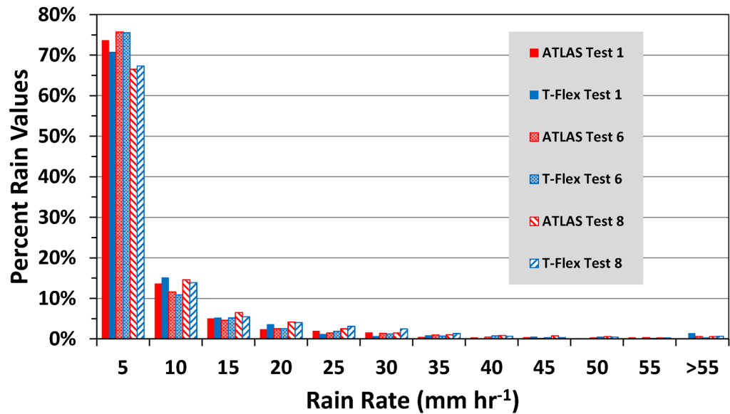
Figure 10. Percentage distribution of rain rate observations by intensity (mm hr -1 ). Percentages are relative to the total number of rain rate observations above 0.4 mm hr -1 . ATLAS data are in red and T-Flex data in blue.
