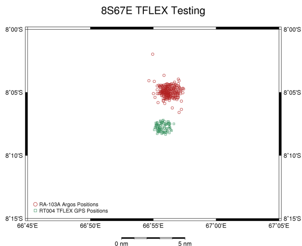
Figure F1. Mooring locations reported by Argos (ATLAS RA103) and GPS (T-Flex RT004).
