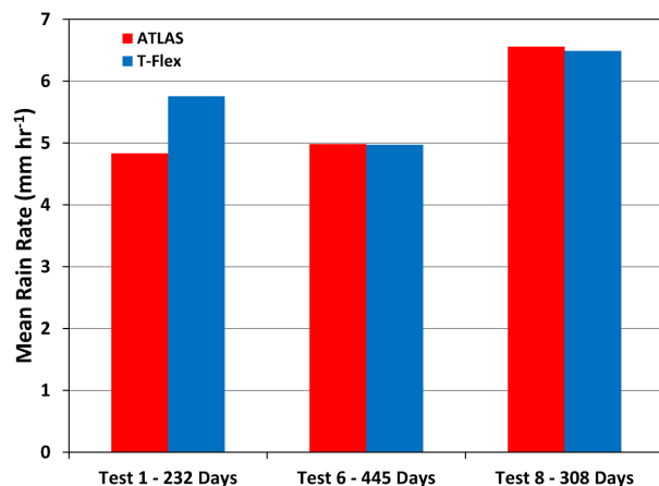
Figure 12. ATLAS (red) and T-Flex (blue) mean rain rates for Tests 1, 6, and 8.
