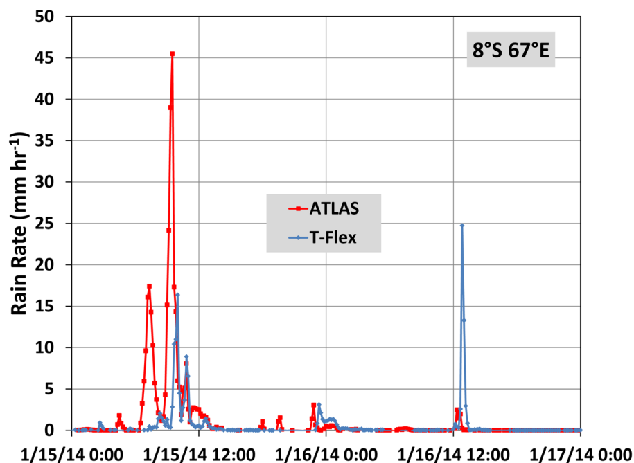
Figure 9. Test 6 10-min rain rate from ATLAS (red) and T-Flex (blue) gauges on 15–16 January 2014. The moorings were separated by 3.2 nm.
