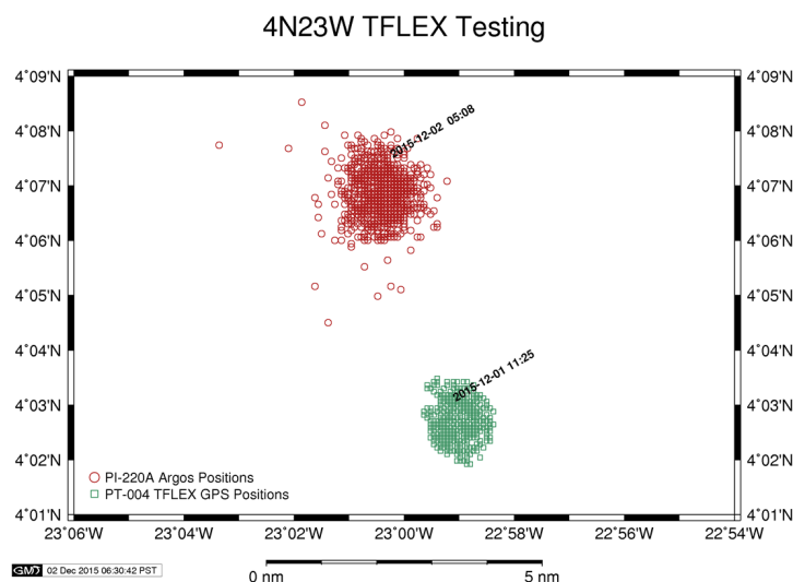
Figure H1. Mooring locations reported by Argos (ATLAS PI220) and GPS (T-Flex PT004).
