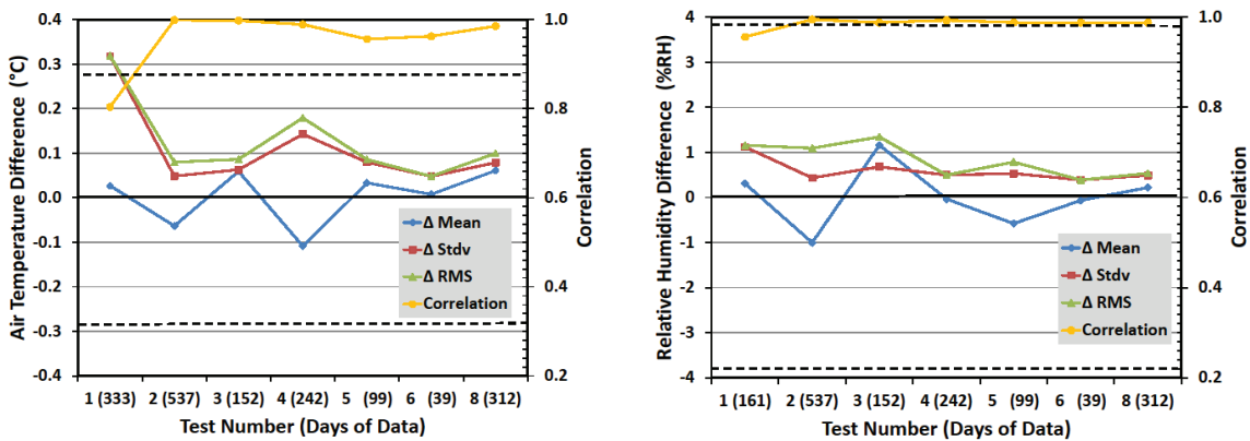
Figure 5. Mean (blue), standard deviation (red), and RMS (green) difference and correlation coefficients ( R^2 , yellow) between T-Flex and ATLAS daily mean air temperature (left) and relative humidity (right). Dashed lines indicate expected maximum difference under the assumption that ATLAS and T-Flex sensor accuracies are comparable. The numbers of daily mean values per test are in parenthesis on the x axis.
