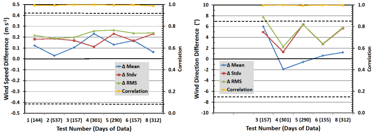
Figure 7. Mean (blue), standard deviation (red), and RMS (green) difference and correlation coefficients (R2, yellow) between T-Flex and ATLAS daily mean wind speed (left) and wind direction (right). Dashed lines indicate expected maximum difference under the assumption that ATLAS and T-Flex sensor accuracies are comparable. The numbers of daily mean values per test are in parenthesis on the x axis.
