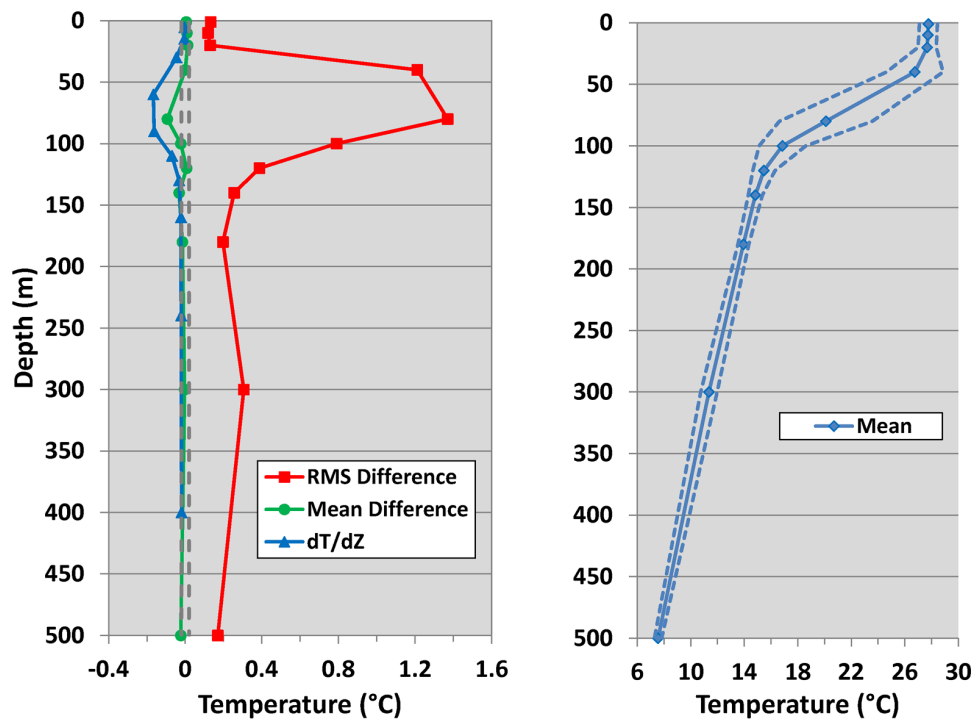
Figure 14. Left: Test 8 T-Flex PT004 minus ATLAS PI220 mean (green) and RMS (red) temperature difference. Mean ATLAS dT/dZ (blue). Right: ATLAS mean temperature profile (solid blue), and mean \pm standard deviation (dashed blue).
