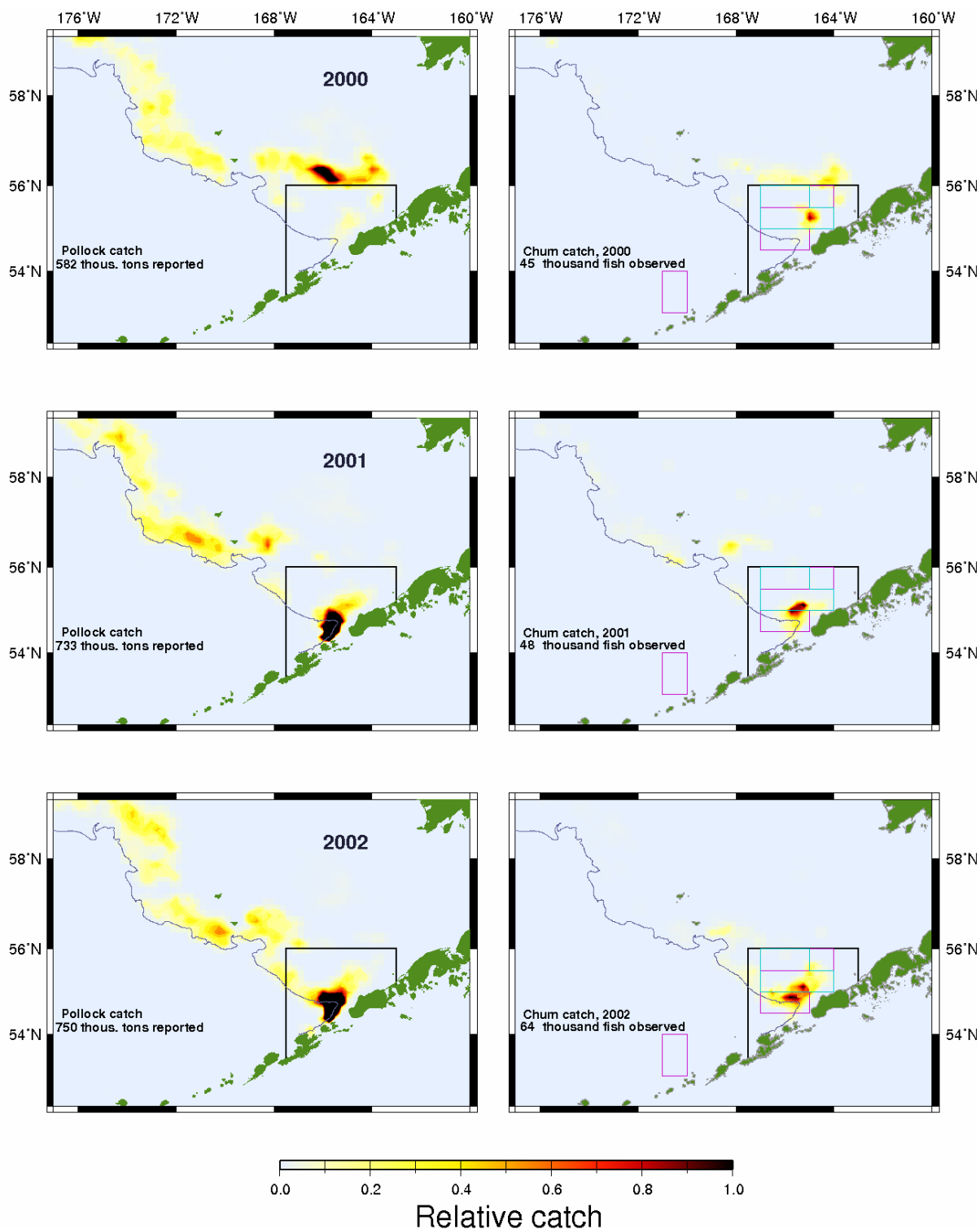
Figure 4-19 Pollock catch during the "B" season (June – Dec; left column) compared to non-chinook (labeled as chum) salmon catch for the same period (right column). Source: NMFS Observer database. The scale of the relative catch is constant for each species over different years.
