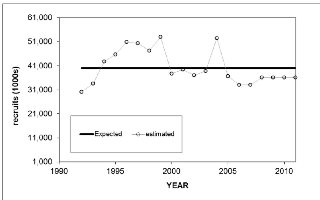
Figure 73. Time series of expected recruitment (in thousands of age 0 fish), with the time series of individual year class estimates predicted by the model and the expected Beverton-Holt stock-recruit relationship with a steepness of 1.0.
