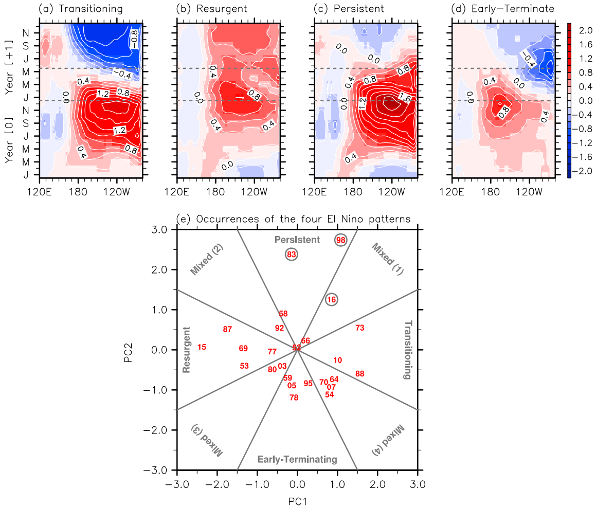
Figure 2. (a–d) Time-longitude plots of the tropical Pacific SSTAs, averaged between 5°S and 5°N, illustrate the four most frequently recurring El Niño patterns during 1948–2016, namely, (a) the transitioning, (b) resurgent, (c) persistent, and (d) early-terminating El Niño. (e) Normalized PC1 versus PC2 values for all 25 El Niño events. The two digit numbers indicate the El Niño decay years. The dashed gray lines in Figures 2a–2c indicate January 1(+1) and May 31(+1). The thick gray lines in Figure 2e are the boundaries (i.e., PC1 = \pm 2 \times PC2 and PC2 = \pm 2 \times PC1 ) that separate the four El Niño flavors from the mixed flavors. The units for SSTAs in Figures 2a–2d are in °C.
