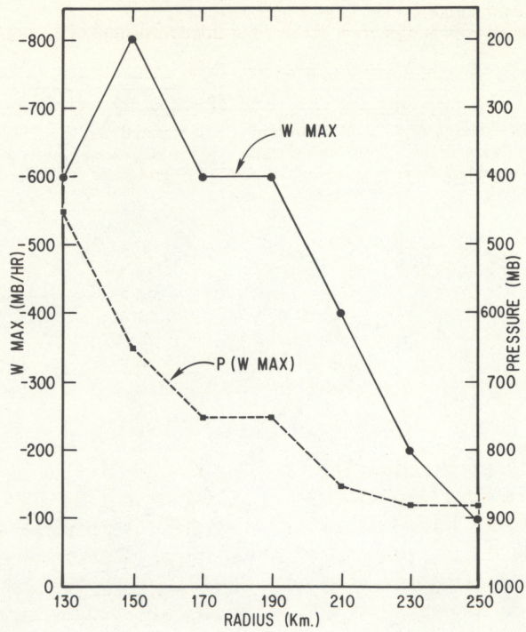
Figure 47.—Data from Exp. 20. Abscissa is the radius at which clouds formed between 10:00 h and 24:00 h. Left ordinate is maximum vertical motion \omega (=dp/dt) that occurred in that cloud during its lifetime (solid curve). The right ordinate is the height (base-state pressure) at which that maximum vertical motion occurred (dashed curve).
