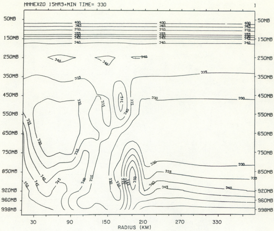
Figure 41.—Vertical cross section of moist static energy at 20:30 h (Exp. 20).
