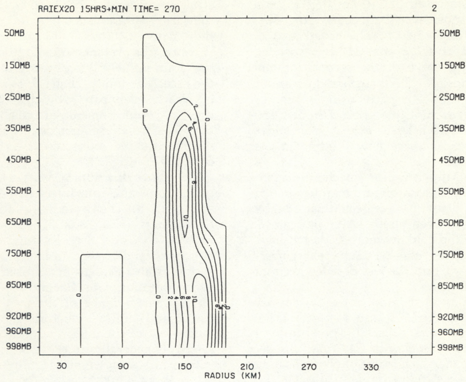
Figure 39.—Vertical cross section of rainwater at 19:30 h (Exp. 20).
