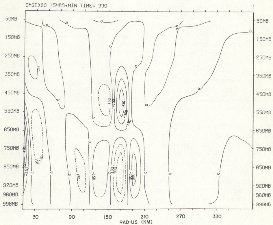
Figure 40.—Vertical cross section of \omega at 20:30 h (Exp. 20).
