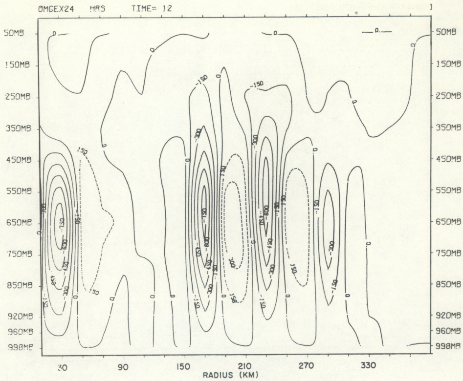
Figure 55.—Vertical cross section of \omega at 12:00 h (Exp. 24).
