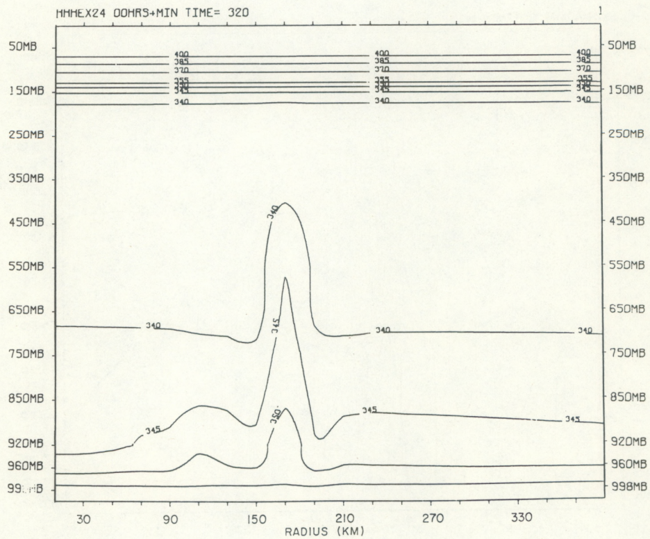
Figure 56.—Vertical cross section of moist static energy at 5:20 h (Exp. 24).
