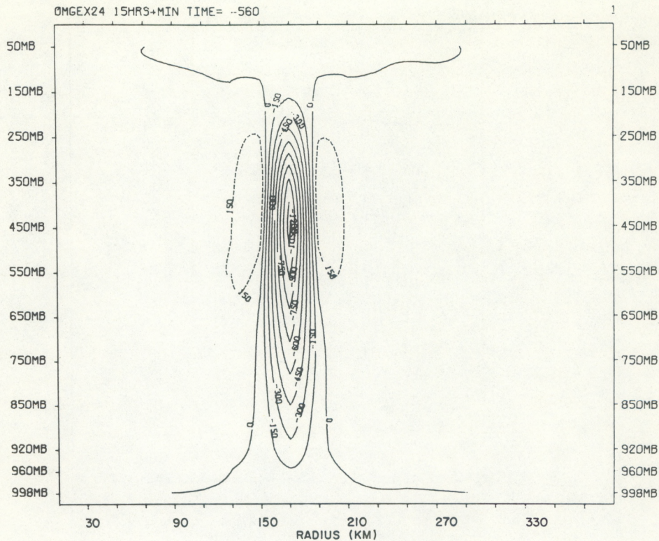
Figure 52.—Vertical cross section of \omega at 5:40 h (Exp. 24).
