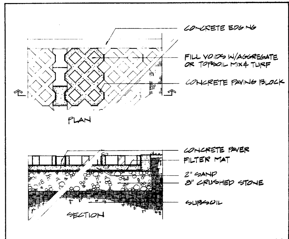
lattice block paving
