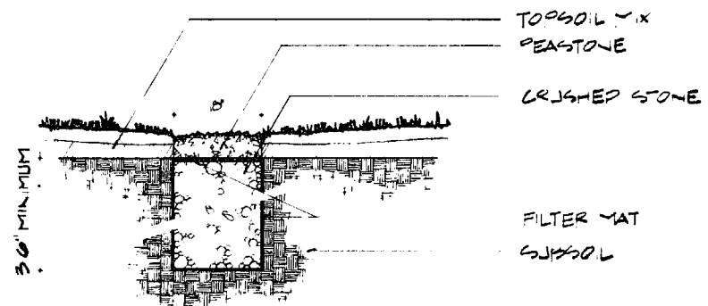
infiltration pit/trench
