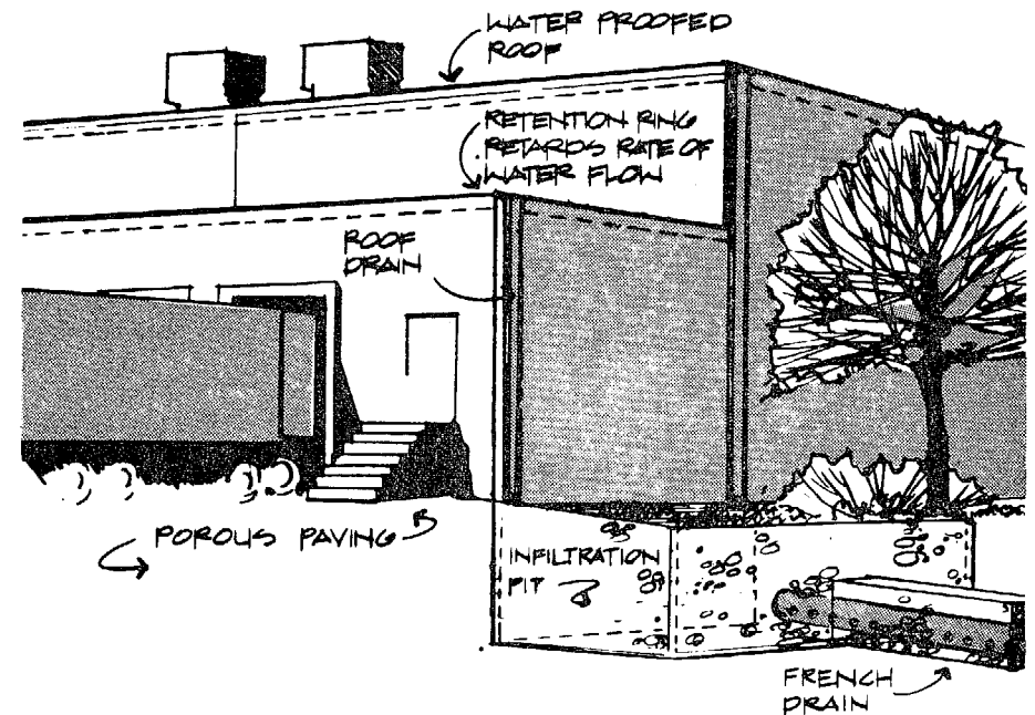
rooftop drainage system
