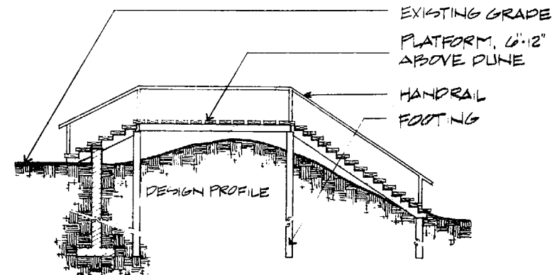
dune walkover
