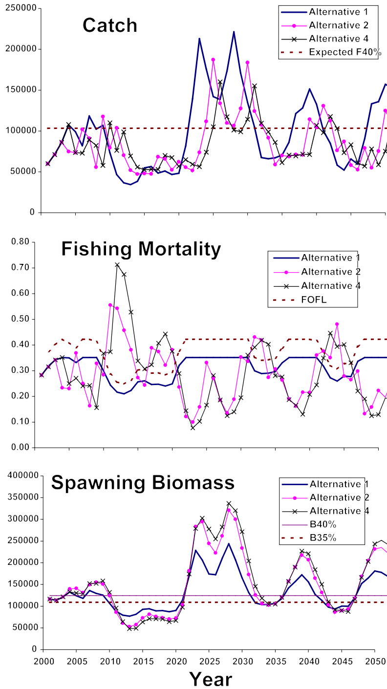
Figure 4.6 Simulated Aleutian Islands atka mackerel trajectory showing the first 50 years of catches (top), fishing mortality rates (middle) and spawning biomass under different alternatives relative to some reference points. Catch and biomass are in metric tons.
