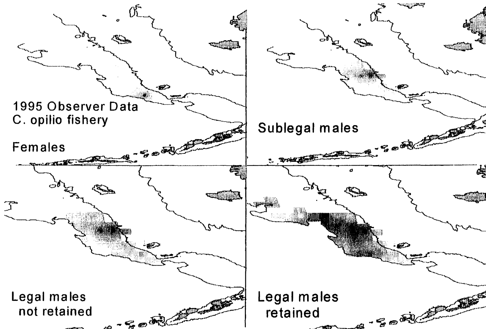
Figure 30 Z-score surfaces of mean CPUE for C. opilio from the Bering Sea 1995 C. opilio fishery. Data is from 1,529 pots sampled by observers on 17 catcher processors participating in the fishery.
