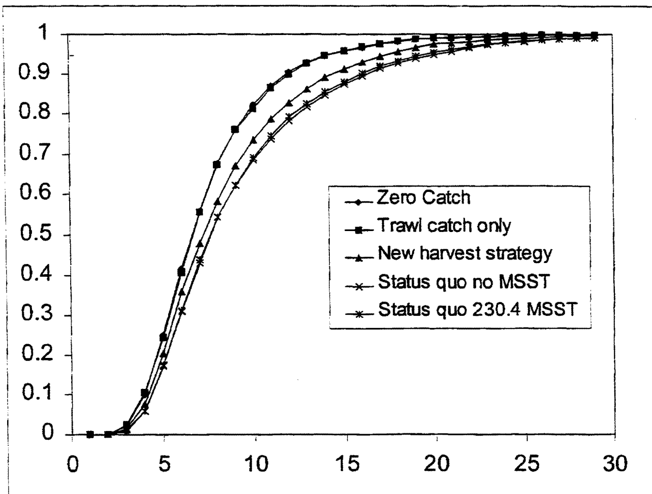
Figure 38 Probability of rebuilding by year for various catch scenarios with random recruitment. Year 1 corresponds to year 2000.
