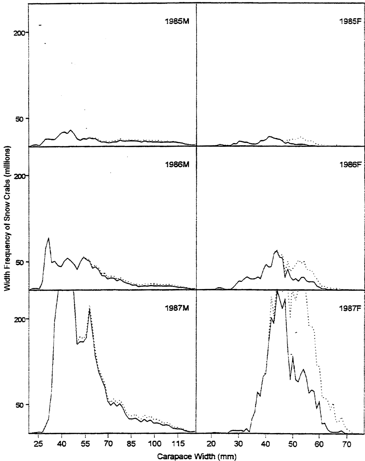
Figure 6 Comparison of width frequency of male (M) and female (F) snow crab abundance south of 61.2°N in the eastern Bering Sea from 1985 to 1987. Solid lines—newshell male or immature female crabs, and differences between dotted and solid lines—oldshell male or mature female crabs.
