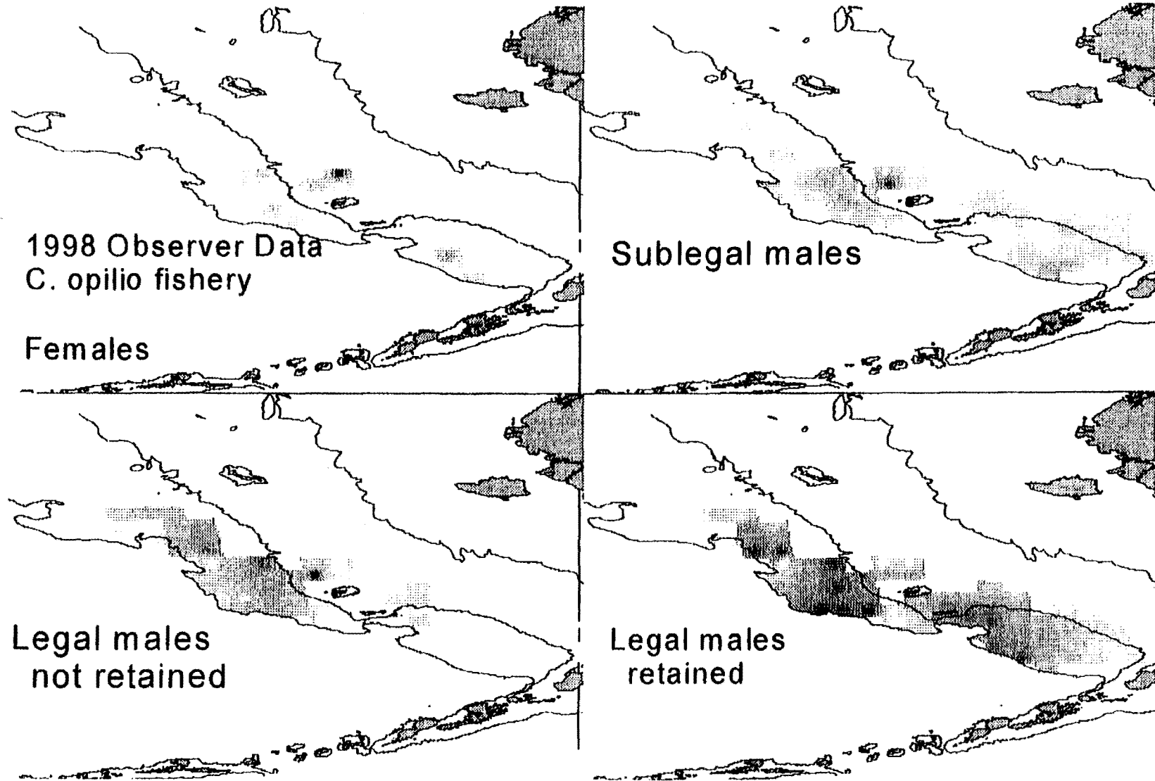
Figure 33 Z-score surfaces of mean CPUE for C. opilio from the Bering Sea 1998 C. opilio fishery. Data is from 1,782 pots sampled by observers on 10 catcher processors participating in the fishery.
