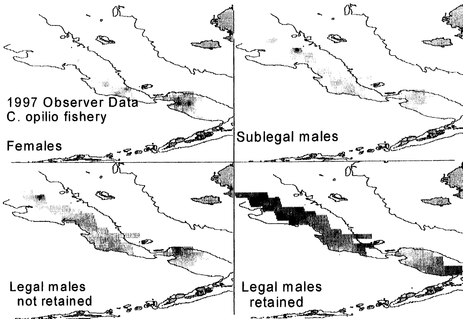
Figure 32 Z-score surfaces of mean CPUE for C. opilio from the Bering Sea 1997 C. opilio fishery. Data is from 1,733 pots sampled by observers on 13 catcher processors participating in the fishery.
