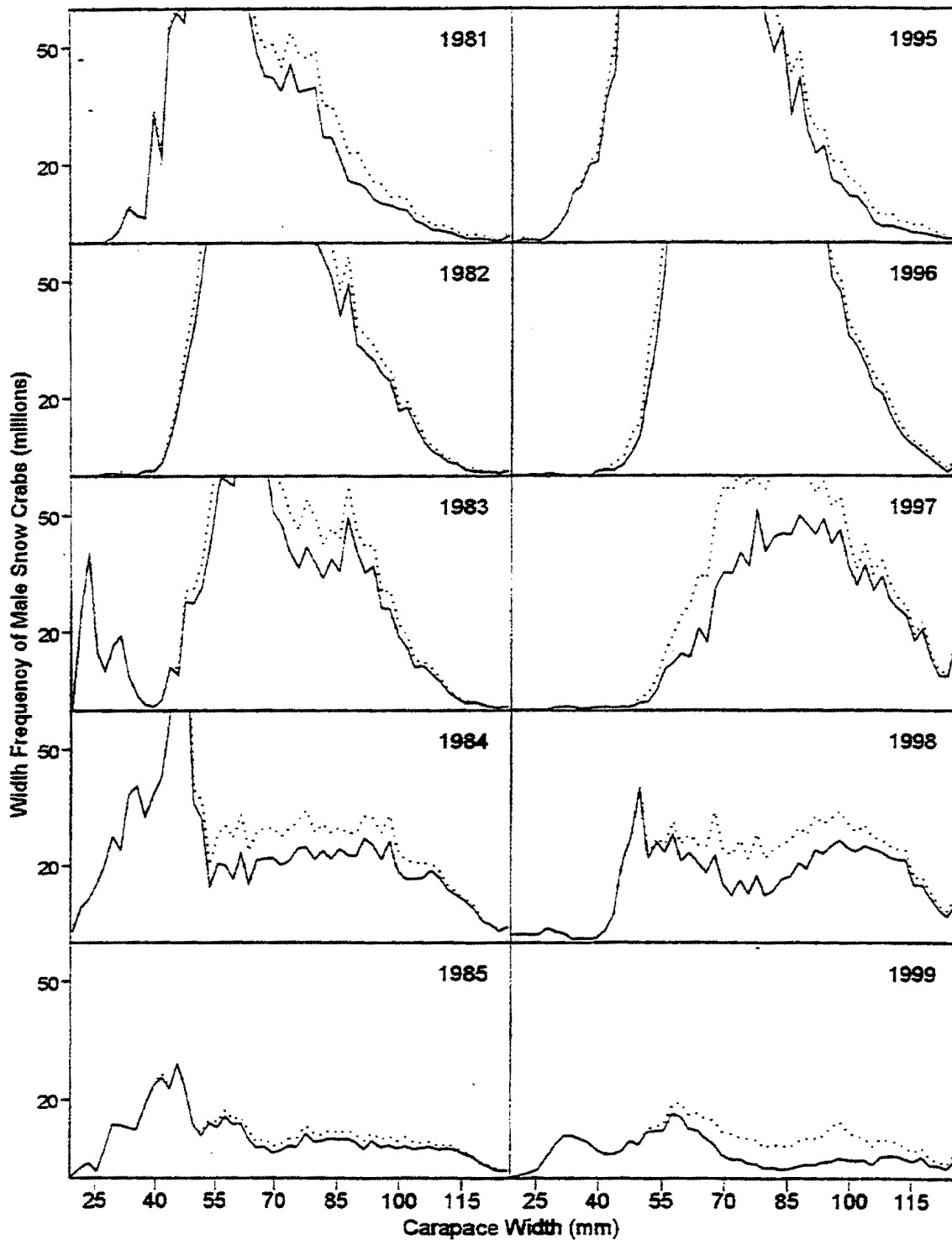
Figure 4 Comparison of width frequency of male snow crab abundance south of 61.2^{\circ}\text{N} in the eastern Bering Sea from 1981 to 1985 and from 1995 to 1999. Solid lines—newshell crabs, and differences between dotted and solid lines—oldshell crabs.
