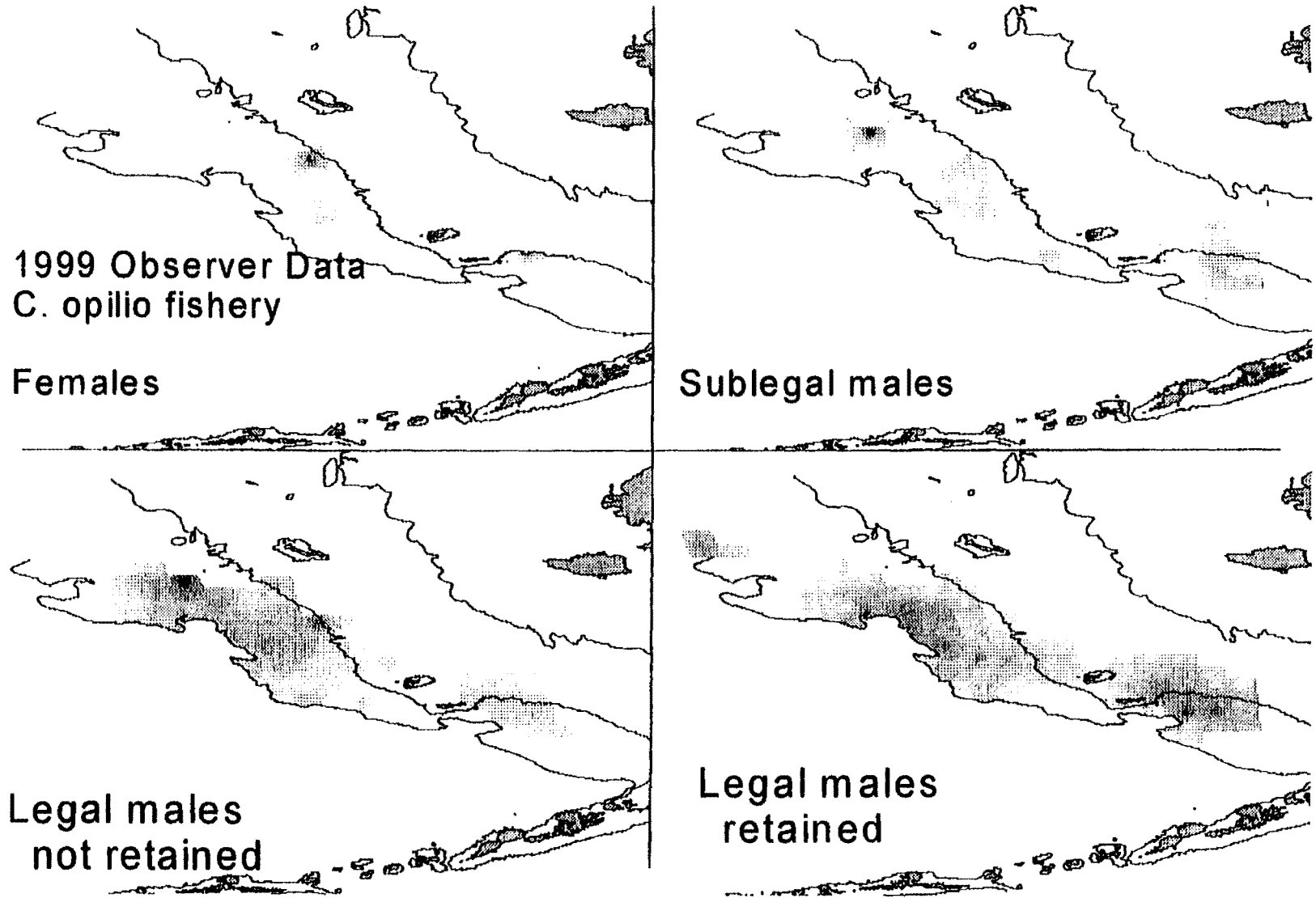
Figure 34 Z-score surfaces of mean CPUE for C. opilio from the Bering Sea 1999 C. opilio fishery. Data is from 1,506 pots sampled by observers on 10 catcher processors participating in the fishery.
