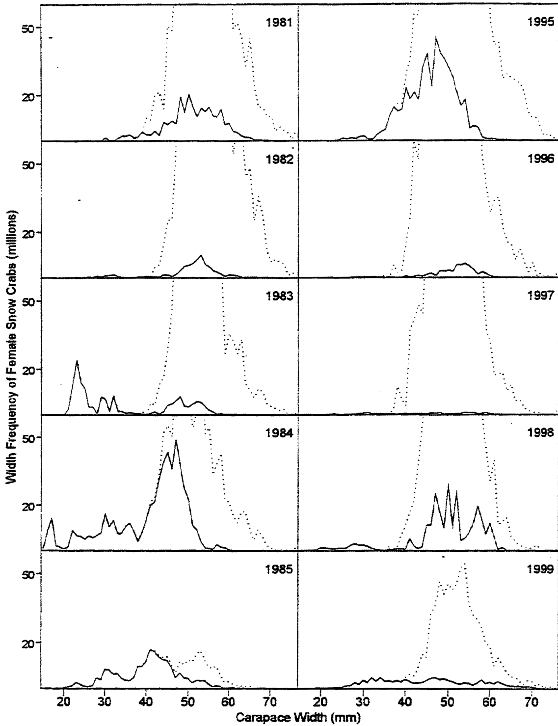
Figure 5 Comparison of width frequency of female snow crab abundance south of 61.2°N in the eastern Bering Sea from 1981 to 1985 and from 1995 to 1999. Solid lines — immature crabs, and differences between dotted and solid lines—mature crabs.
