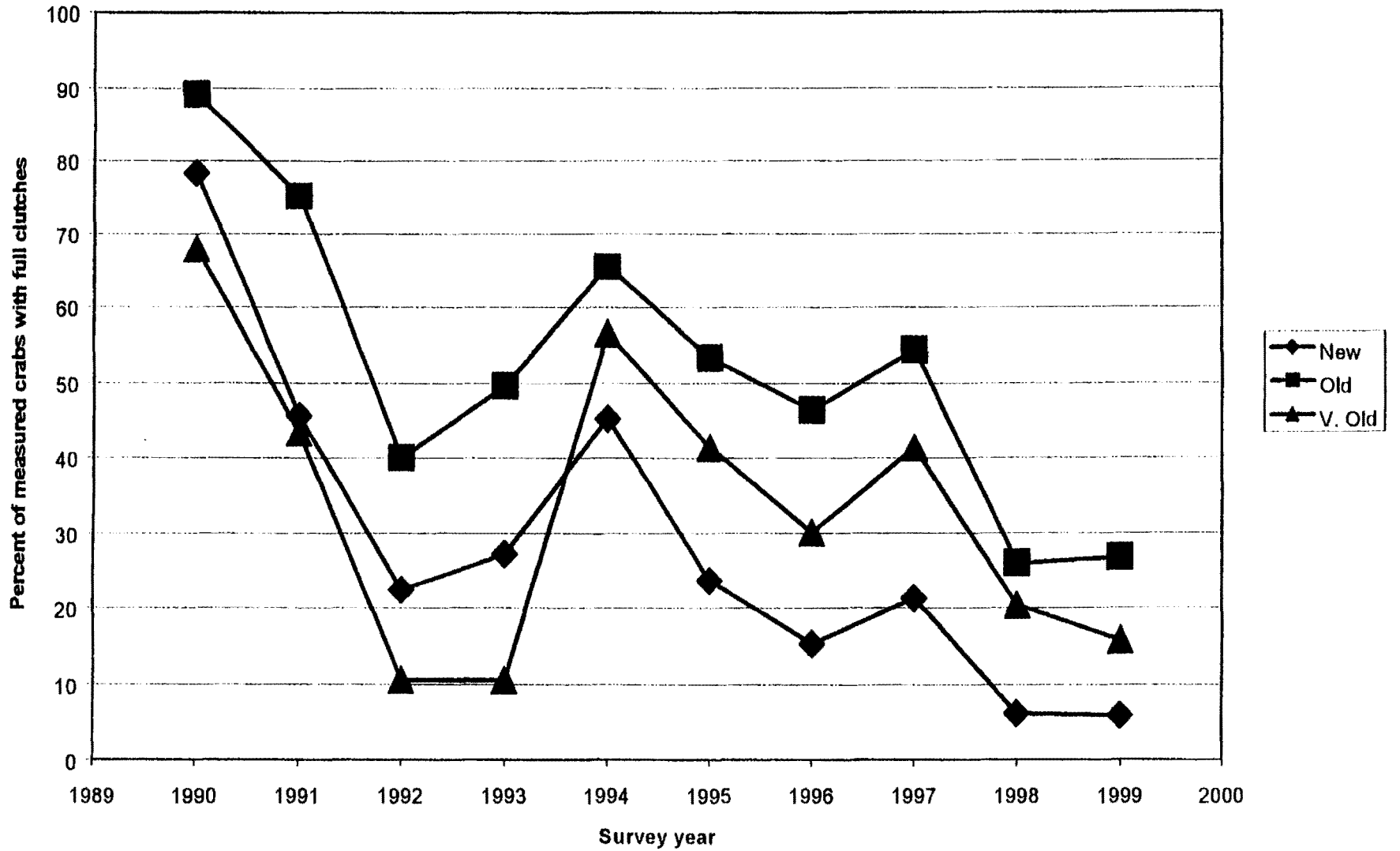
Figure 8 Incidence of full clutches in mature female EBS snow crab by shell age: 1990-1999
