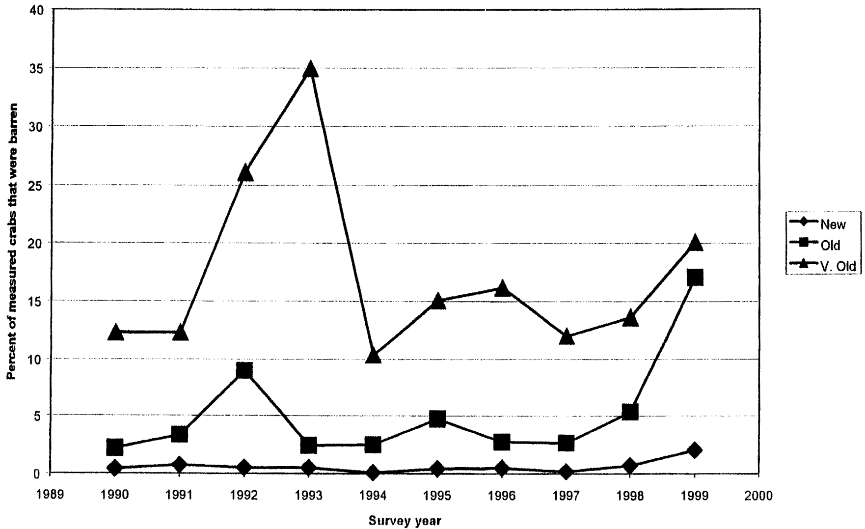
Figure 7 Incidence of barren mature female EBS snow crab by shell age: 1990-1999
