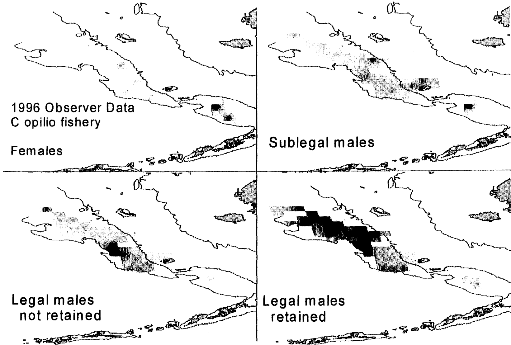
Figure 31 Z-score surfaces of mean CPUE for C. opilio from the Bering Sea 1996 C. opilio fishery. Data is from 1,384 pots sampled by observers on 15 catcher processors participating in the fishery.
