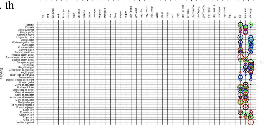
Figure 10. Summary of variable importance across all variables, species, and seasons modeled. a) np component; b) mu component; c) theta component. For complete set of variable importance plots, see Appendix H.
