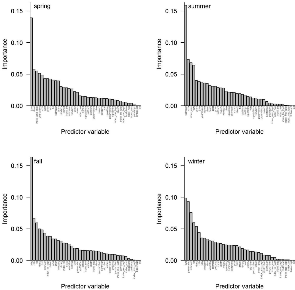
Figure 12. Variable importance for mu model component: average importance of each variable calculated over all final selected models in each season. Note that average importance values have been sorted in descending order for each season, so that the order of variables along the x-axis varies from season to season. Also note that the species modeled in each season, and therefore the species included in the average for each seasonal panel of this plot, vary as shown in Table 2. For complete set of variable importance plots, see Appendix H.
