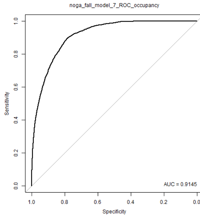
Figure 7.2. Receiver Operating Characteristic (ROC) curves for assessment of predictive accuracy of example model 7 (NOGA/fall). a) ROC curve and area under the curve (AUC) statistic for prediction of median-thresholded non-zero data (i.e., non-zero data above/below median observed value), b) ROC curve and AUC statistic for prediction of presence/absence. For complete set of ROC curves for selected models, see Appendix F. For complete set of AUC statistics for selected models, see Table 11.
