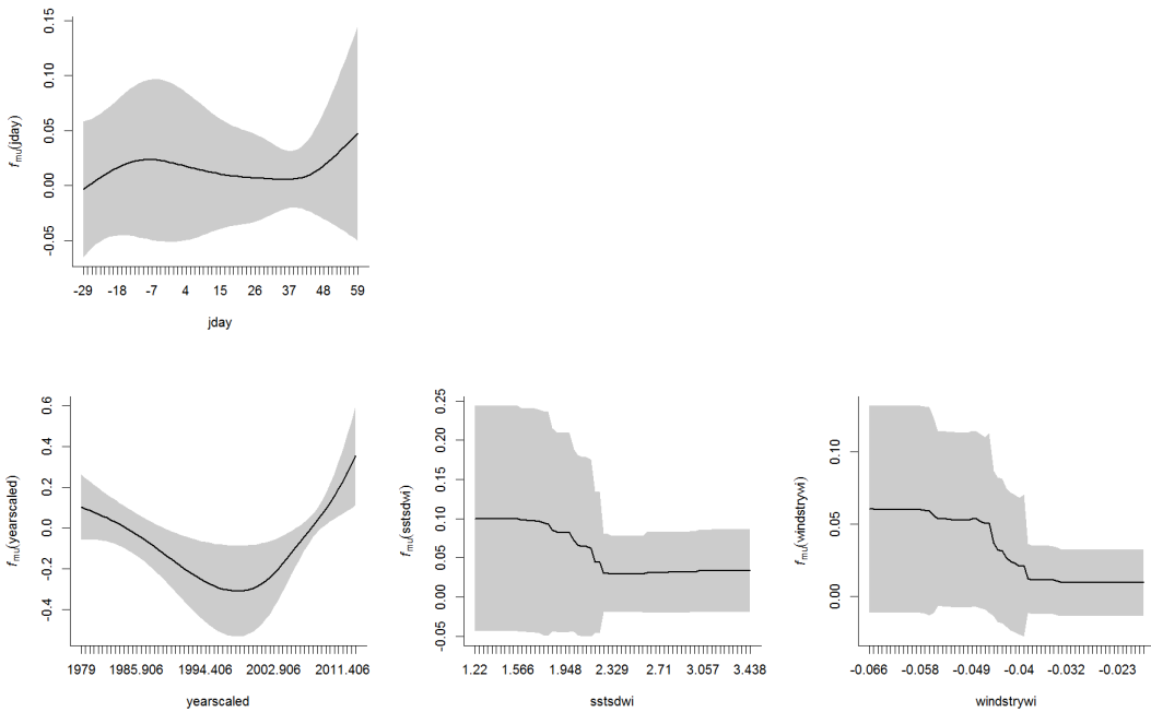
Figure 14.3. Selected bootstrap marginal plots for example model 7 (RAZO/winter). Solid line is bootstrap mean and grey shading indicates +/- 1 bootstrap standard deviation. a) np component of model b) mu component of model. Full sets of marginal plots in Appendix I.
