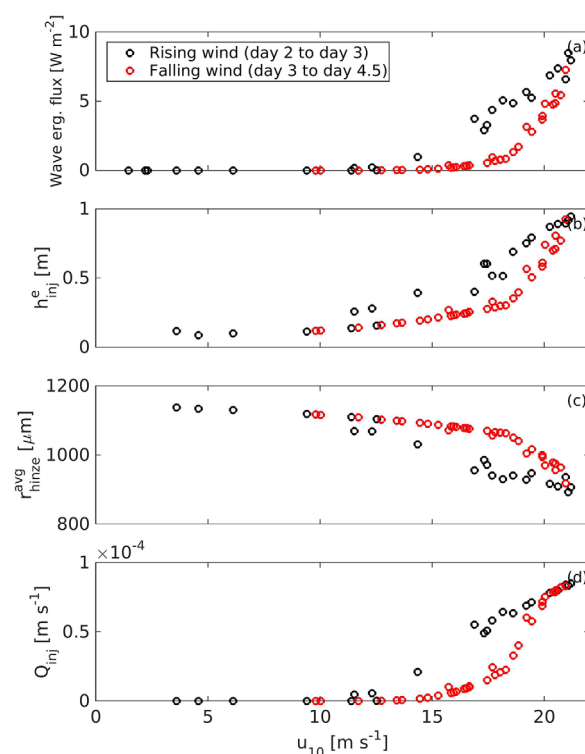
Figure 10. (a) Wave energy flux ( \mathcal{E} ) calculated using Terray's relation [Terray et al. , 1996] during rising and falling wind; (b) e-folding depth of injected air using the breaking wave model by Sullivan et al. [2007] during rising and falling wind; (c) Hinze scale weighted averaged by injected air amount during rising and falling wind; and (d) the rate of injected air during rising and falling wind.
