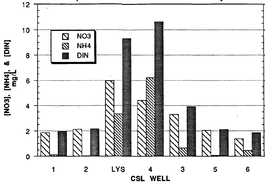
FIGURE 25A SITE CSL Mean N-species Concentrations in Wells & Lysimeter
