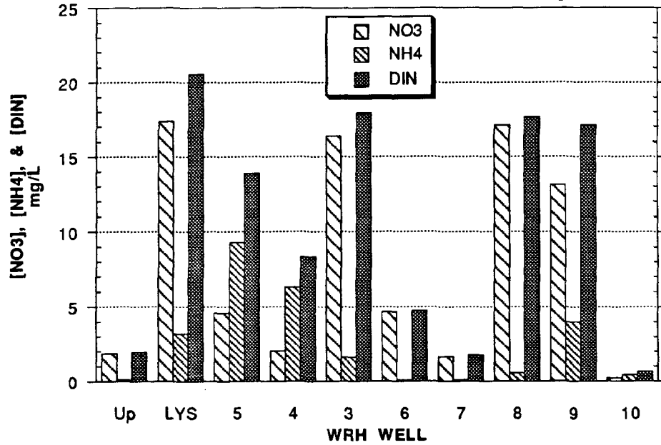
FIGURE 24A SITE WRH Mean Nutrient Concentrations in Wells and Lysimeter
