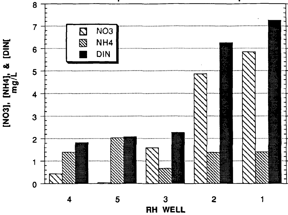
FIGURE 30A SITE RH Mean N-species in Well Water Samples
