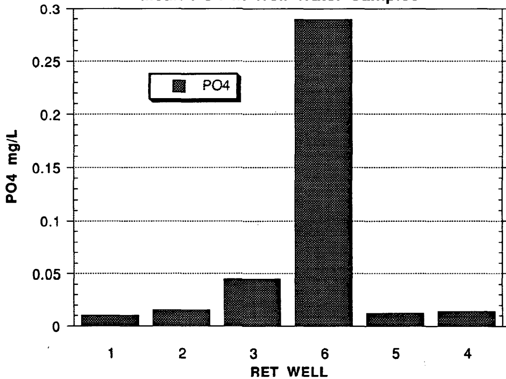
FIGURE 28B SITE RET Mean PO4 in Well Water Samples
