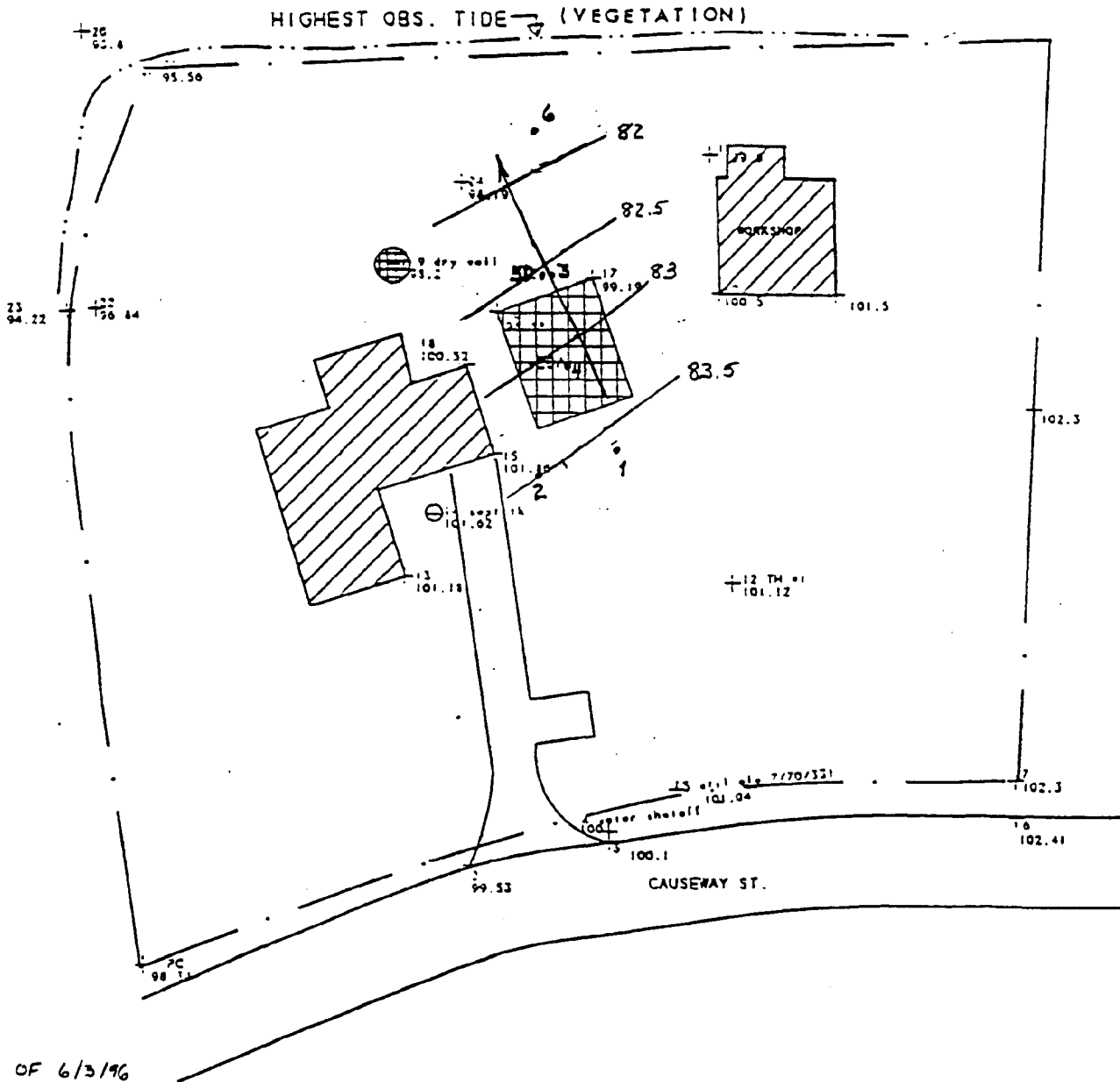
Figure 19. Groundwater flow directions at site CSL: 6/3/96.
