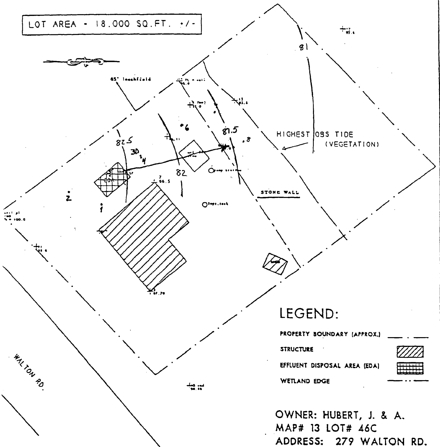
Figure 18. Groundwater flow directions at site WRH: 6/6/96.
