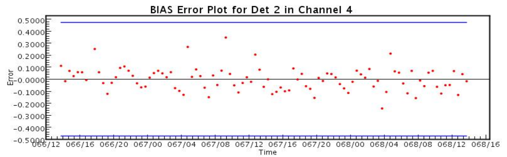
Figure 2 The errors for GOES 13 channel 4 detector 2. The blue lines are the outlier threshold, which is defined as 5 times of the noise level \sigma_e obtained from the ATLMA training. The x-axis is the time with the convention of <DAYOFTHEYEAR>/<HOUROFTHEDAY>.
