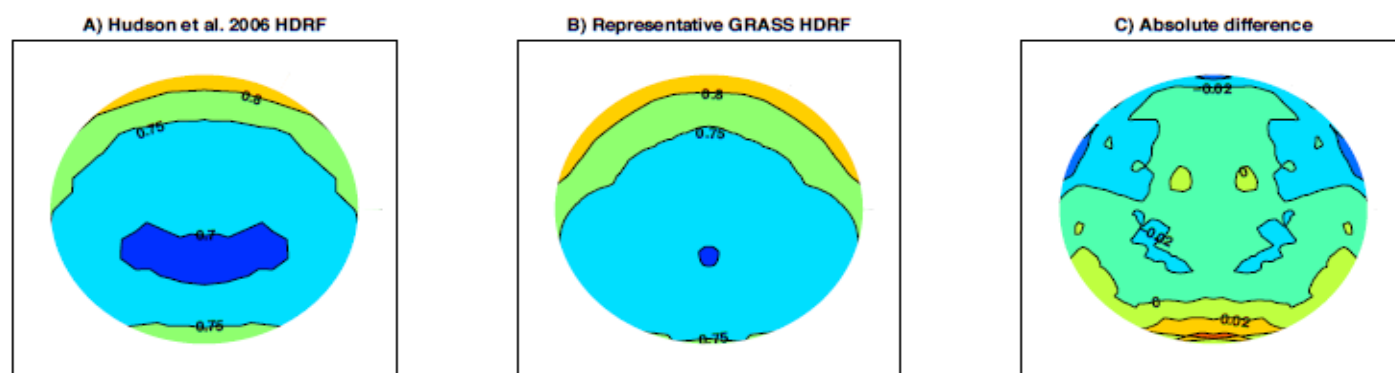
Figure 2: Comparison between HDRF measurements by Hudson et al. (2006) compared to HDRF measurements with GRASS at 1000 nm, taken at similar solar zenith angles. The solar principle plane runs vertically from the top to bottom of the plots.
